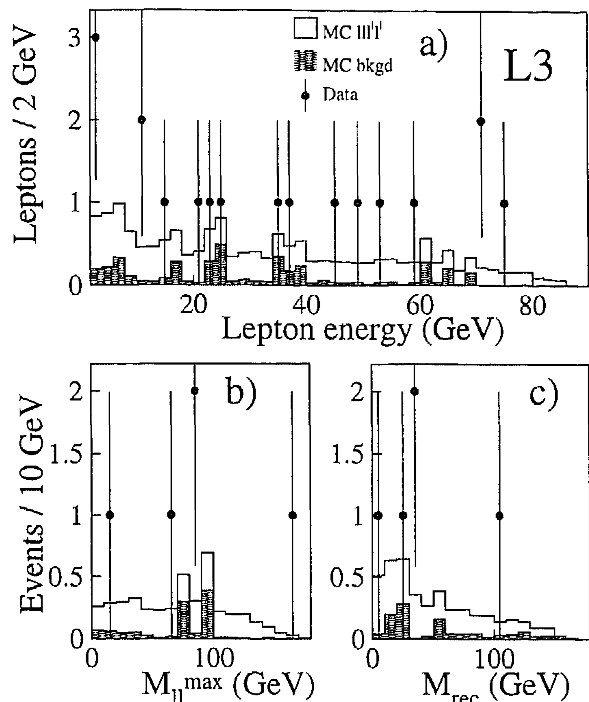
Fig. 2. Distributions for the low-multiplicity selection ( ll' ll' ) of (a) the lepton energy, (b) the highest lepton-pair invariant mass per event for leptons of the same flavour and (c) the corresponding recoil mass. The open histograms are the Monte Carlo predicted four-fermion distributions, the hatched histograms are the Monte Carlo predicted background distributions and the points are the data events.
