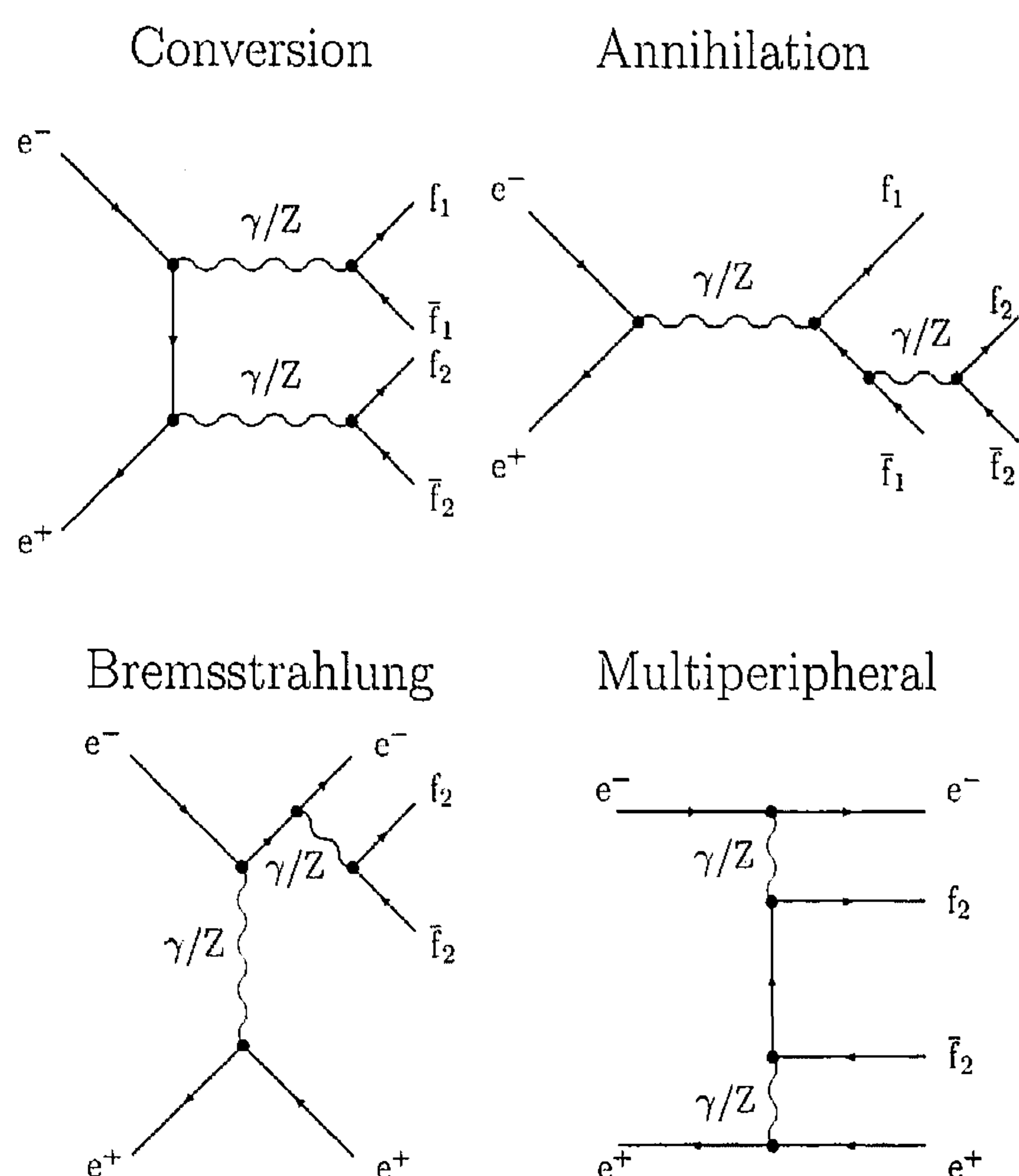
Fig. 1. The lowest-order Feynman diagrams for the process e^+e^- \rightarrow f_1\bar{f}_1f_2\bar{f}_2 .
