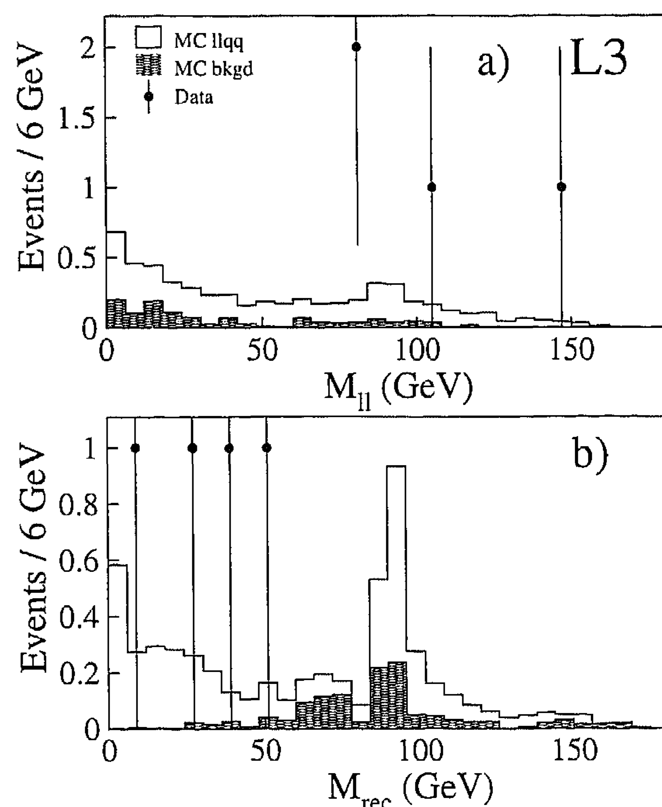
Fig. 3. Distributions for the high-multiplicity selection ( llqq ) of (a) the lepton-pair invariant mass and (b) the their recoil mass. The open histograms are the Monte Carlo predicted four-fermion distributions, the hatched histograms are the Monte Carlo predicted background distributions and the points are the data events.
