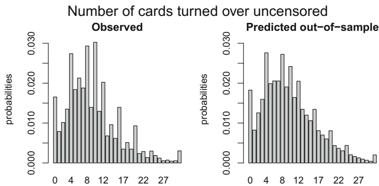
FIGURE 10. Distribution of the empirical (left panel) and predicted number of cards turned over by the CMM (right panel) for the uncensored observations in the test data.
