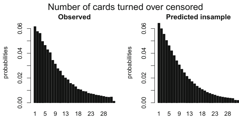
FIGURE 9. Distribution of the empirical (left panel) and predicted by the CMM (right panel) number of cards turned over corrected for the probability of being censored per card in the training data.
