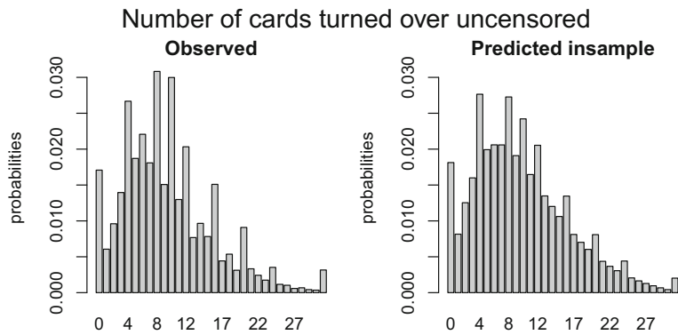
FIGURE 8. Distribution of the empirical (left panel) and predicted by the CMM (right panel) number of cards turned over for the uncensored observations in the training data.
