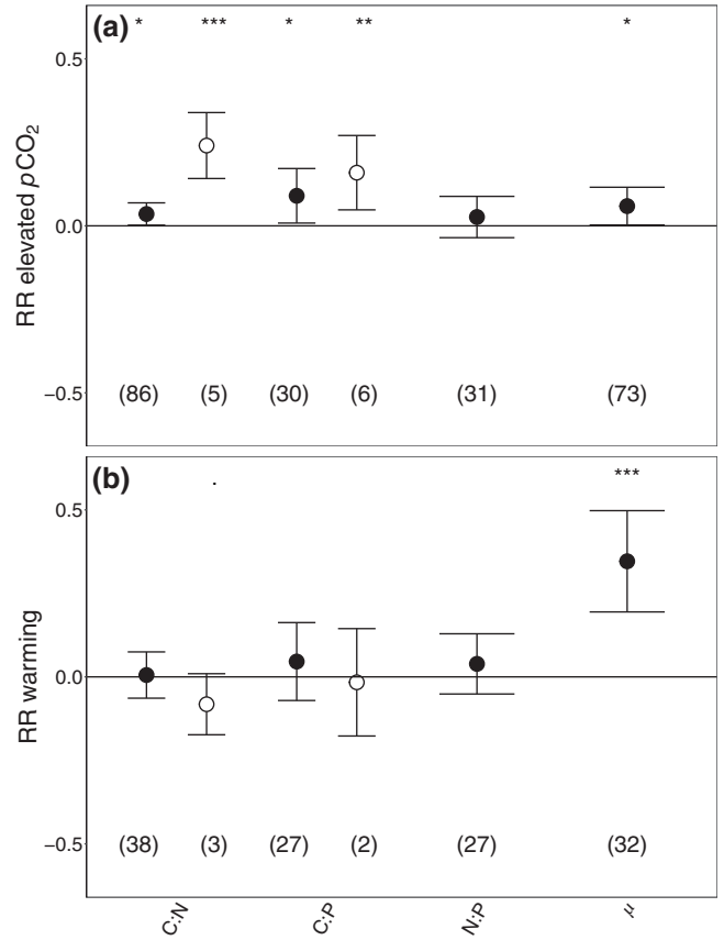
Fig. 1. Natural-log response ratios of elevated p\text{CO}_2 (a) and warming (b) on the C:N, C:P, and N:P ratios and growth rate ( \mu ) of marine phytoplankton under nutrient-replete (closed circles), nitrogen- (open circles for C:N), and phosphorus-limited (open circles for C:P) conditions. Error bars represent 95% confidence intervals and sample sizes are between brackets and Significance levels are indicated as follows: *** p < 0.001 , ** p < 0.01 , * p < 0.05 , p < 0.10 .
