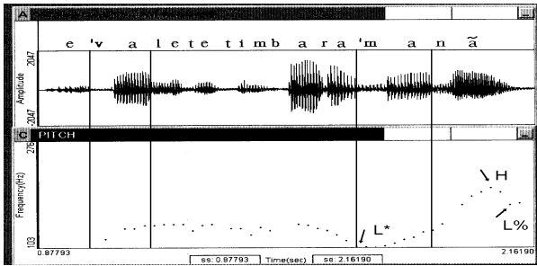
Figure 1: Waveform and F_0 contour of the test sentence [⊙⊙⊙⊙⊙⊙⊙⊙⊙⊙⊙⊙⊙⊙⊙⊙⊙⊙⊙⊙⊙⊙⊙⊙] 'Put-past-pl. the-safety-pin' "Did you put the SAFETY-PIN?" by speaker KR. The vertical lines delimit the two stressed syllables of the utterance.
