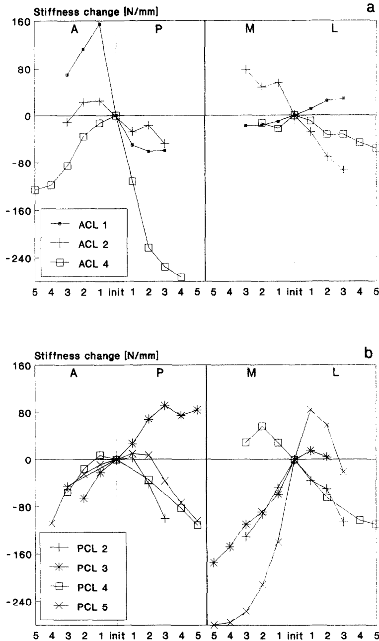
Fig. 5. The absolute stiffness change ( N\ mm^{-1} ) from the initial orientation (init.) to the tilted positions 1–5 for each tilt direction (Fig. 3) of the anterior cruciate ligaments (a) and the posterior cruciate ligaments (b). A: anterior; P: posterior; M: medial; L: lateral; init.: initial orientation of the bones.
