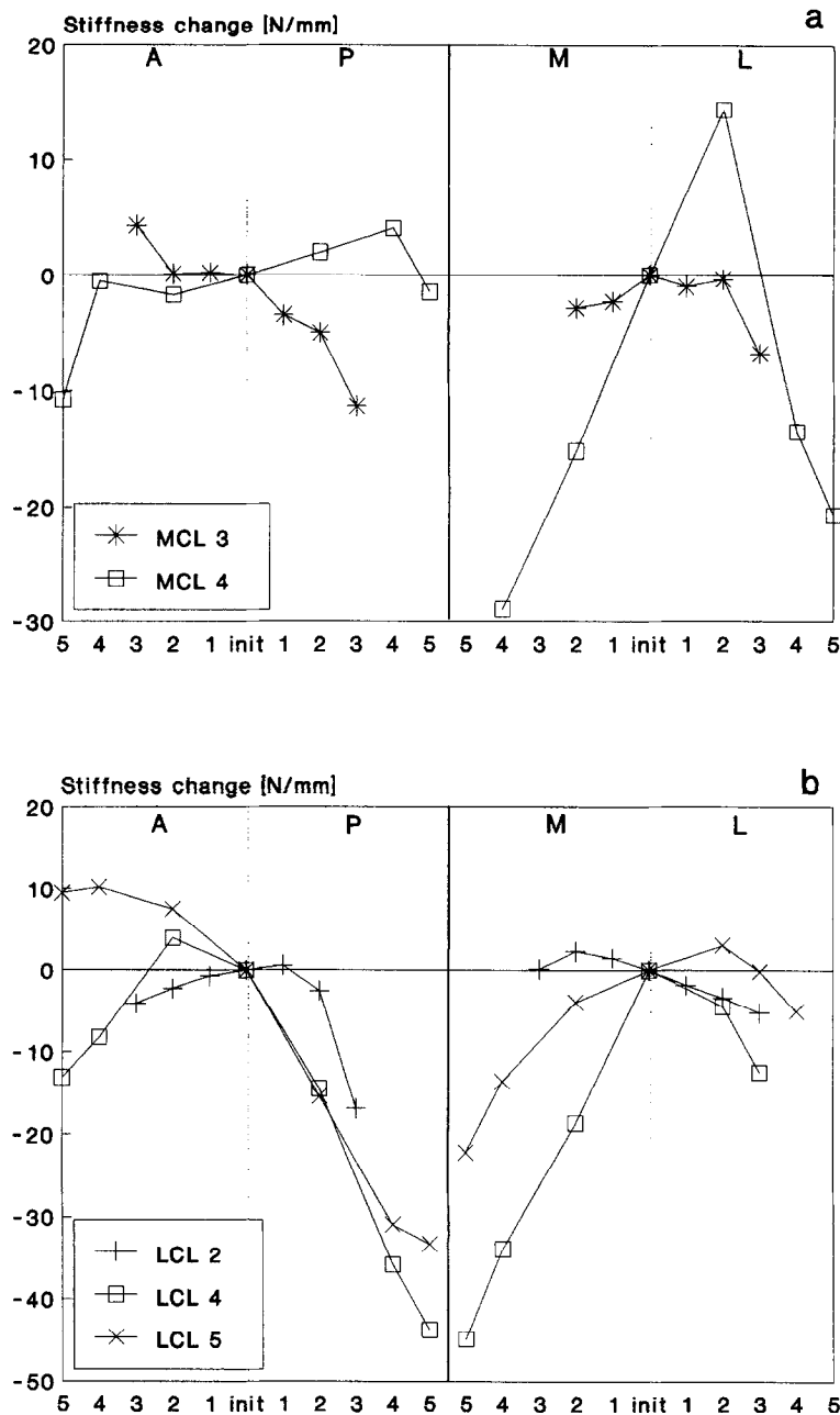
Fig 6. The absolute stiffness change ( \text{N mm}^{-1} ) from the initial orientation (init.) to the tilted positions 1–5 in each tilt direction (Fig. 3) for the medial collateral ligaments (a) and the lateral collateral ligaments (b). Note that the scale of the y-axis has been changed in comparison to Fig. 5. A: anterior; P: posterior; M: medial; L: lateral.
