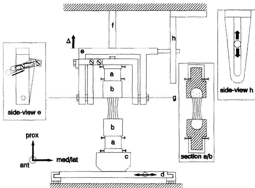
Fig. 2. Two-dimensional schematic representation of a bone-ligament-bone preparation fixed in a loading rig in a material testing machine. (a) Fixation pots, (b) part of the PMMA block (hatched) containing the bones with the tantalum pellets, (c) load cell, (d) X-Y table, (e) tilting device, (f) actuator, (g) tilting axis, (h) conductor.
