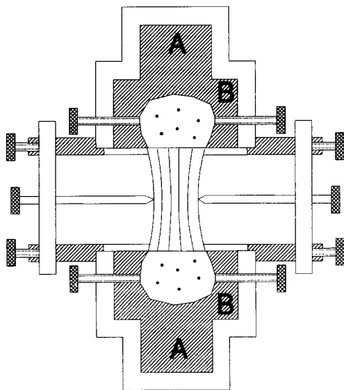
Fig. 1. Schematic representation showing a cross-section of a bone–ligament–bone preparation, with in the bones the 0.5 mm pellets, fixed in a mold. This mold is specially designed to position the insertion sites of the ligament in the mold center as best as possible and to tense the ligament fibers as uniformly as possible in the initial orientation. When this was achieved, the bones were potted in two-tier polymethylmethacrylate (A and B).
