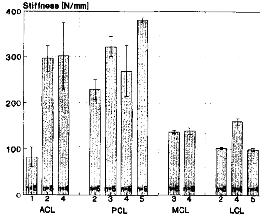
Fig. 4. The average ( \pm standard deviation) of the stiffnesses ( N mm^{-1} ) measured in the initial orientations of the bone-ligament-bone preparations of the anterior cruciate ligaments (ACL), the posterior cruciate ligaments (PCL), the medial collateral ligaments (MCL) and the lateral collateral ligaments (LCL) of knee specimens 1-5 (x-axis). n = the number of initial orientations.
