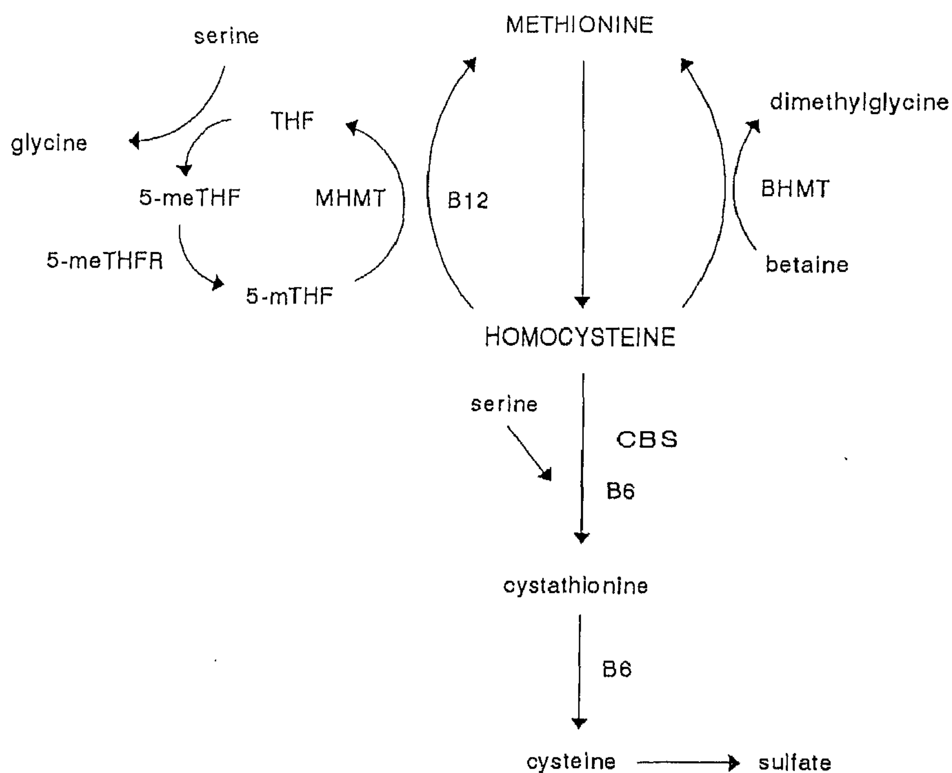
Fig. 1. The main reactions in methionine and homocysteine metabolism by transsulphuration and remethylation. MH = 5,10-methyltetrahydrofolate-homocysteine methyltransferase (methionine synthase); BH = betaine-homocysteine methyltransferase; 5-meTHFR = 5-methylenetetrahydrofolate reductase; CBS = cystathionine \beta -synthase; 5-mTHF = 5-methyltetrahydrofolate; 5-meTHF = 5-methylenetetrahydrofolate; B 6 = pyridoxal 5'-phosphate (from vitamin B 6 ).
