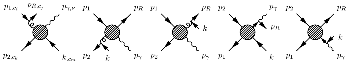
Figure 8. NLO Feynman diagrams for the NLP contributions of the process q(p_1)\bar{q}(p_2) \rightarrow q(p_R)\bar{q}(k)\gamma(p_\gamma) .
