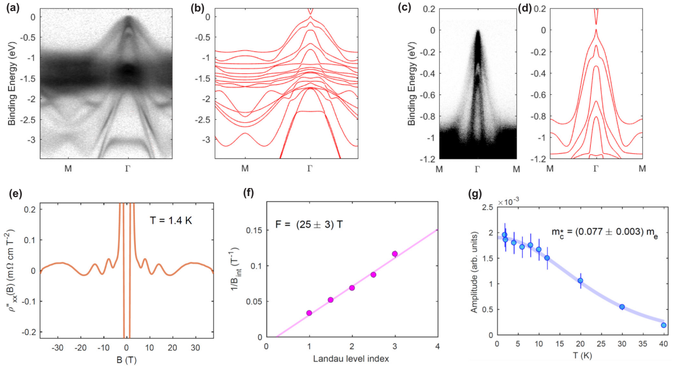
FIG. 3. ARPES and high-field magnetotransport of \text{EuCd}_2\text{As}_2 . (a), (c) ARPES spectrum as a function of wave vector along the M - \Gamma - M high-symmetry line measured at T \simeq 5 K with incident photon energy of 130 eV. The data shown here are a sum of two measurements taken with linear-vertical and linear-horizontal polarization, respectively, to compensate the effect of selection rules. Nonlinear scaling was applied to the intensity to enhance the visibility of bands with a small photoemission cross section. (b), (d) Electronic bands calculated by DFT (in red). (e) The second derivative of the longitudinal resistivity \rho''_{xx}(B) as a function of field applied along the c axis. (f) Plot of 1/B_{\text{int}} at the minima and maxima in \rho_{xx} against Landau level index, with integers assigned to the minima, where B_{\text{int}} = B + \mu_0 M is the internal field. The Shubnikov–de Haas (SdH) frequency F is obtained from the gradient of the linear fit shown. (g) Temperature dependence of the amplitude in the SdH oscillation, measured at B = 10 T. The line is a fit to the Lifshitz-Kosevich formula, from which the cyclotron effective mass m_c^* of the charge carriers is estimated. The quoted error in m_c^* derives from the least-squares fit, but the uncertainty in the measurement is expected to be larger because of the long period of the oscillations and the relatively narrow field range.
