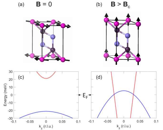
FIG. 2. Exchange-induced Weyl nodes in \text{EuCd}_2\text{As}_2 . (a), (c) In zero field, the Eu spins order in an A -type antiferromagnetic structure at T < T_N , with the spins lying in the ab plane. The corresponding band structure is gapped at \Gamma , and every band is doubly degenerate due to the combination of inversion and time-reversal symmetries. (b), (d) The Eu moments can be fully polarized along the c axis in a small coercive field ( B > B_c ), lifting the double degeneracy of the bands and creating a pair of Weyl nodes along \Gamma - A , at k_z = 0.03 r.l.u.
