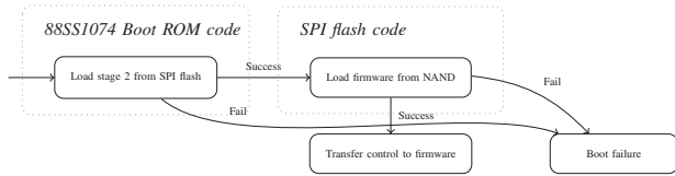
Fig. 1. Crucial MX300 boot process.
