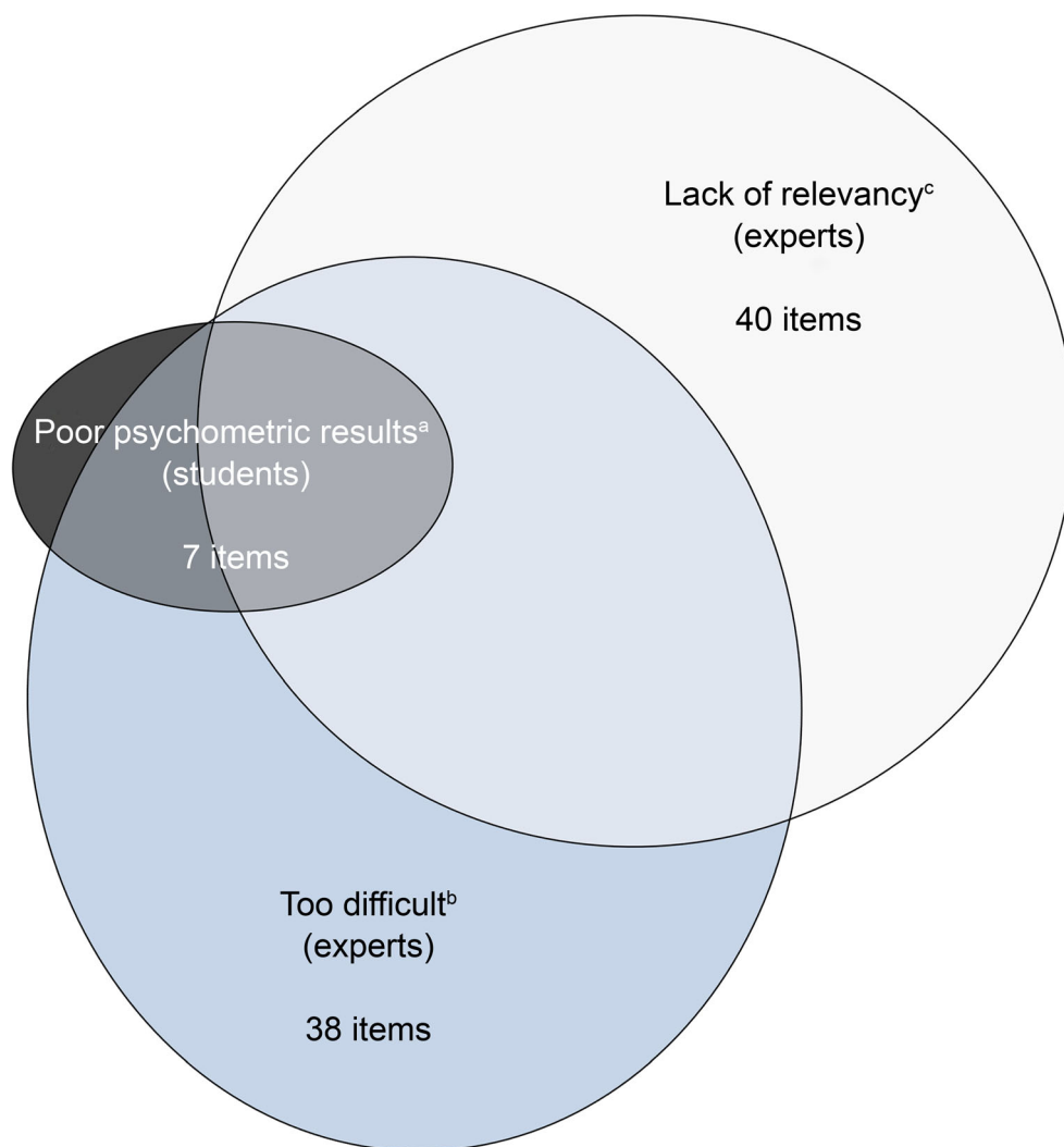
Fig. 1 Diagram of items for revision ordered by selection criterion. Additional 52 items selected for revision based on expert criteria in addition to classic test analysis criteria' from students' results. a Poor psychometric results indicating that students who overall did poorly on the test did better on that item than did students who overall did well ( p value < 0.65 for students and item-rest-correlation \leq 0 ). b Too high difficulty for the experts (difficulty index: p' < 0.8 ), c Lack of relevancy as rated by the majority of the content expert panel
