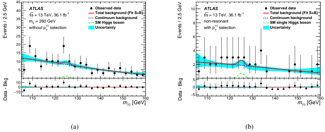
Figure 3: Invariant mass spectrum of the diphoton system in the searches for both resonant and non-resonant Higgs boson pair production, with the corresponding backgrounds for (a) m_X = 260 GeV without any p_T^{\gamma\gamma} selection and (b) the non-resonant case with a p_T^{\gamma\gamma} > 100 GeV selection. Fits to m_{\gamma\gamma} are performed using the full signal-plus-background model. In each plot, only the background component is present. The shape parameters and normalisation of the continuum background model are determined in the fits. The “SM Higgs boson” in (a) contains the single-Higgs-boson background and SM di-Higgs-boson background. The band shows the uncertainty of the “Total background” in the upper panel and is calculated by a sampling method. The bottom panel shows the difference between the number of events in data and the estimated number of background events, as determined by the fits.
