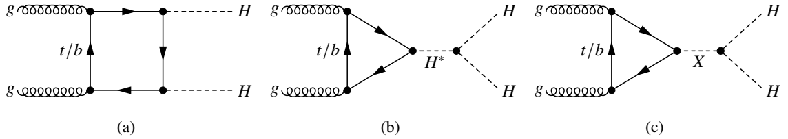
Figure 1: Feynman diagrams for leading-order Higgs boson pair production in the SM through (a) a heavy-quark loop, (b) the Higgs self-coupling, and (c) an intermediate heavy resonance in a BSM scenario. The total SM contribution is the sum of the two modes depicted in (a) and (b), which have significant destructive interference. Physics beyond the SM can enhance Higgs boson pair production either by modifying the Higgs boson coupling constants from their SM values in (a) and/or (b), or by an additional s-channel exchange of an intermediate scalar resonance in (c).
