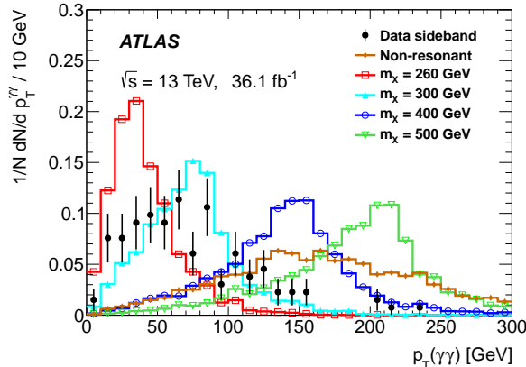
Figure 2: Distributions of the reconstructed transverse momenta of the diphoton system with all event selections, except the p_T^{\gamma\gamma} selection, applied for various signal models, as well as sideband data, normalised to unit area.
