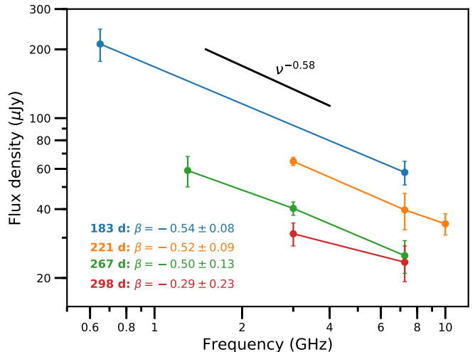
Figure 1. Radio spectral indices between 0.6–10 GHz spanning four epochs observed during the decline part of the light curve. The different epochs are color coded. The approximate number of days post-merger and the corresponding spectral indices are given in the legend. A joint fit to all the radio data implies \beta = -0.53 \pm 0.04 (see §3.2), in good agreement with the radio to X-ray spectral index measurements (shown by the black \nu^{-0.58} line). With this measurement, we can rule out any spectral steepening expected, for example, due to the presence of a cooling break in or between the radio/X-ray bands.
