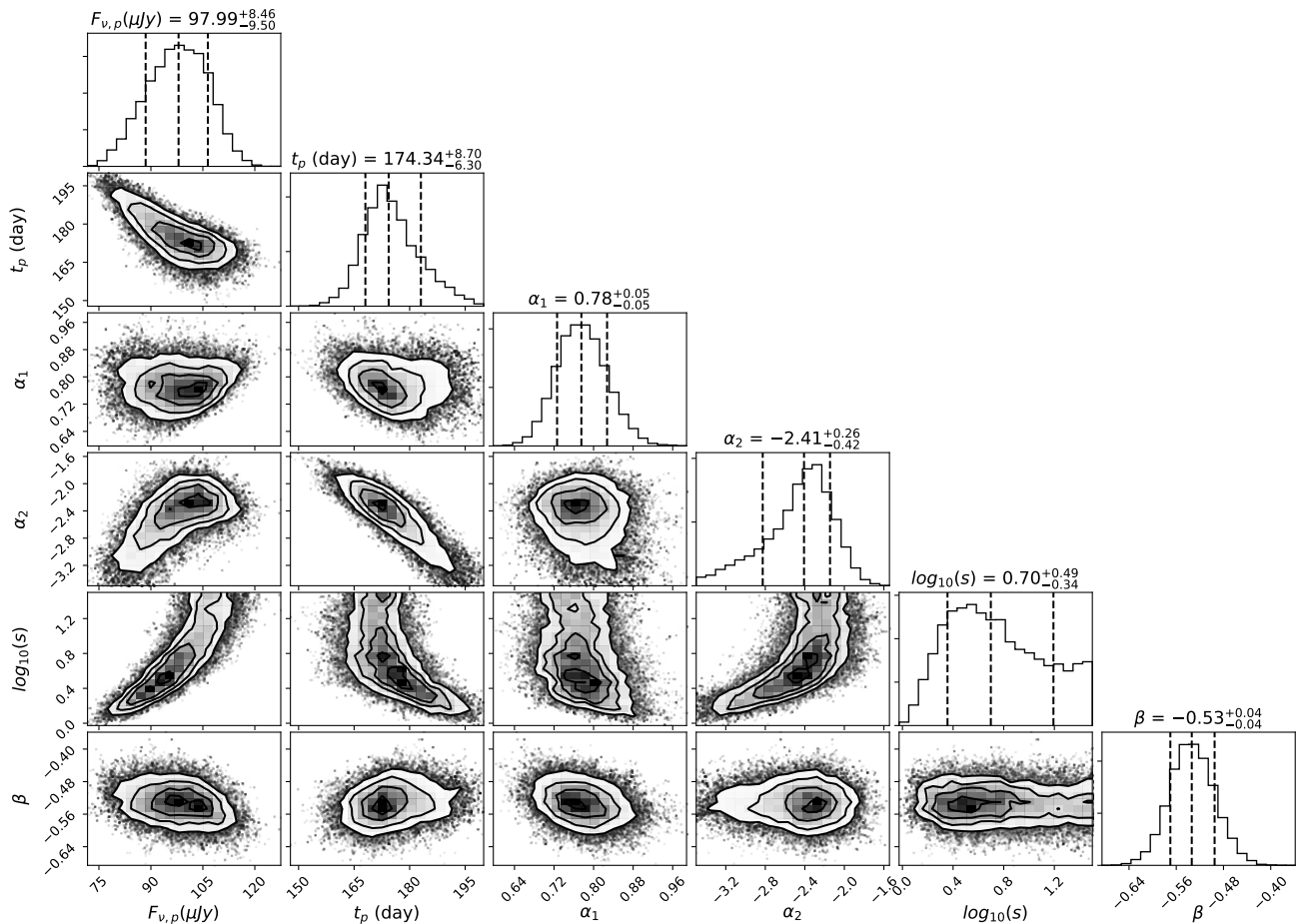
Figure 3. A corner plot showing the results of our MCMC fitting of the radio light curve (Figure 2) using the VLA, ATCA, MeerKAT and uGMRT data. F_{\nu,p} is the flux density at 3 GHz at the time of light curve peak, t_p is the time to light curve peak, \alpha_1, \alpha_2 are the power-law rise and decay slopes, s is the smoothness parameter, and \beta is the spectral index. See §3.2 for details. In each contour plot and histogram, the 16, 50, 84 percentiles are marked.
