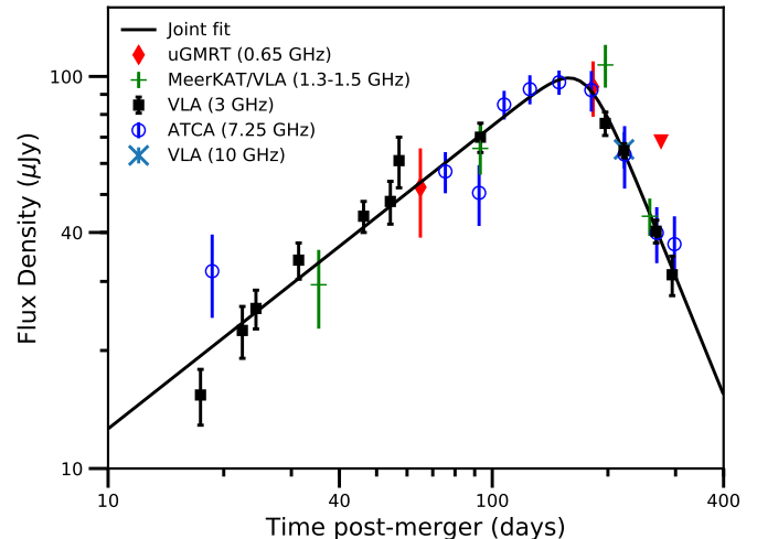
Figure 2. The radio light curve of GW170817 spanning multiple frequencies, and scaled to 3 GHz using the spectral index ( \nu^{-0.53} ) derived from our MCMC analysis. The data from the VLA (filled black squares for 3 GHz and green crosses for 1.5 GHz), the ATCA (blue circles), the MeerKAT (green crosses) and the uGMRT (red diamonds for detections and triangle for upper limit) are as reported in Table 1. We also include the data at 0.65 GHz, 1.5 GHz, 3 GHz, and 7.25 GHz reported previously (Hallinan, Corsi et al. 2017; Mooley et al. 2018a; Dobie et al. 2018). Our best-fit smoothed broken power-law model to all these data (see §3.2) is shown as a solid curve. The power-law decline index obtained is -2.4_{-0.4}^{+0.3} . For comparison, a broken power-law fit to the 3 GHz VLA-only data gives -2.2 \pm 0.2 . Both fits are thus consistent with t^{-p} decline in the light curve, where p is the electron power-law distribution index.
