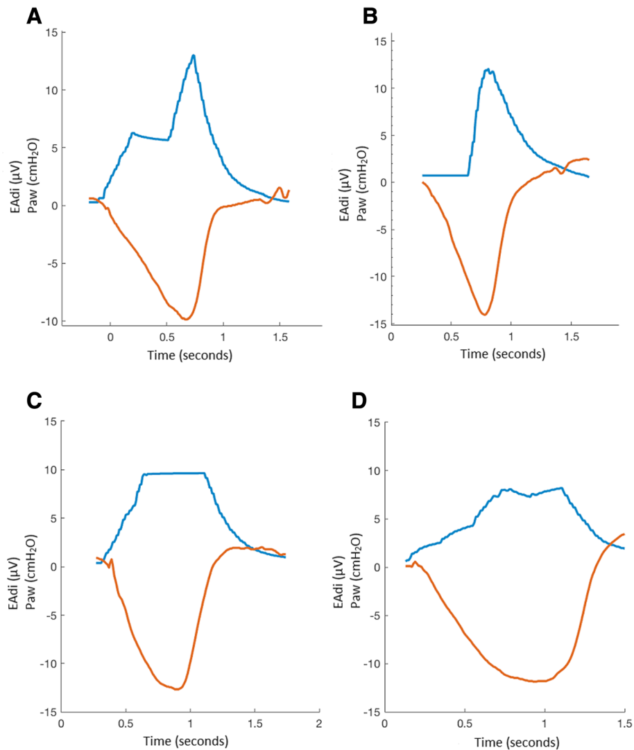
Fig. 3 Four examples of electrical activity of the diaphragm (EAdi) waveform irregularities during an end-expiratory occlusion. The blue line represents the EAdi signal expressed in microvolts. The orange line represent the airway pressure (Paw) expressed in centimeters of water. a Slope < 0 during the ascending part of the EAdi waveform. b Delay in start of EAdi peak. c EAdi peak cut off. d Split EAdi peak
