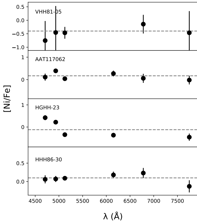
Figure A5. [\text{Ni}/\text{Fe}] abundances as a function of wavelength for a selected sample of GCs in NGC 5128.
