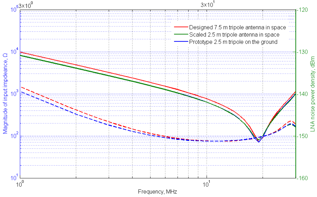
Figure 15: Simulated impedance magnitudes (solid line) and corresponding LNA noises (dashed line) for the proposed 7.5 m tripole antenna, scaled 2.5 m tripole antenna onboard the satellite, and the prototype 2.5 m tripole antenna on the ground. Here the impedance and LNA noise are simulated for 7.5 m antenna at low frequencies (lower) and for 2.5 m antenna at corresponding high frequencies (upper).
