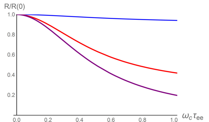
FIG. 3. Resistance in the absence of recombination [Eq. (11b)] in weak magnetic fields. Different curves (top to bottom) correspond to different values of the ratio W/[\ell_G(0)] = 20, 2, 0.2 .
