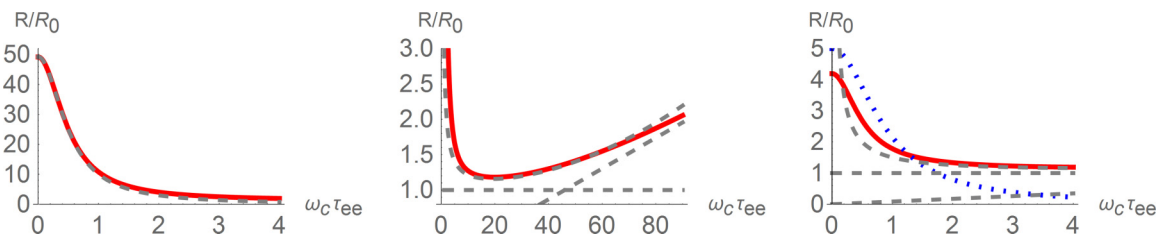
FIG. 6. Intermediate regimes of the resistance. The left panel illustrates the Gurzhi limit in the narrowest samples [Eq. (12)], taking into account higher-order corrections in W/\ell_G(0) = 0.5 while plotting the Lorentzian (dashed curve). The central panel shows Eq. (22) for the same sample width (dashed curve). The numerical values were computed for \ell_R(0)/\ell_G(0) = 120 , \tau\tau_*/\tau_{ee}^2 = 100 . The straight dashed line describes the strong-field limit (21). The right panel shows the onset of the intermediate regime (22) for a wider sample with W/\ell_G(0) = 2 . The dotted line shows the Lorentzian (12).
