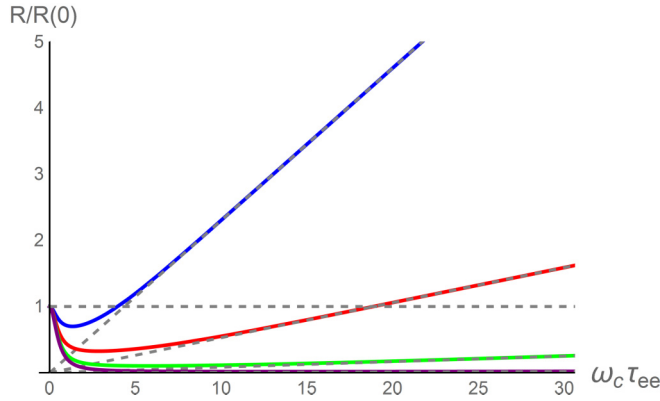
FIG. 7. Nonmonotonic behavior of the resistance (17). Different curves (top to bottom) correspond to different values of the ratio W/[\ell_G(0)] = 4, 2, 1, 0.4 . The numerical values correspond to the choice \ell_R(0)/\ell_G(0) = 50 , \tau\tau_*/\tau_{ee}^2 = 100 . Dashed lines describe the strong-field limit (21).
