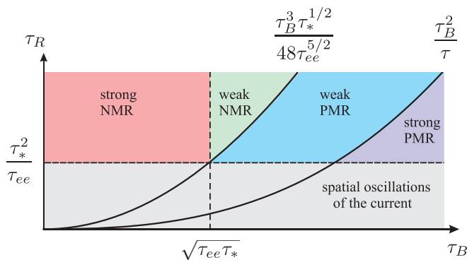
FIG. 8. Summary of the parameter regimes exhibited by the sample resistance subjected to the external magnetic field [Eq. (17)]. The lower part of the diagram with \tau_R \ll \tau_*^2/\tau_{ee} describes the regime where the eigenvalues (14c) are complex and the currents exhibit oscillatory behavior. This regime is beyond the scope of this paper and will be addressed elsewhere. The labels “weak/strong NMR (PMR)” refer to the negative (positive) MR in weak magnetic fields [see Eq. (20)].
