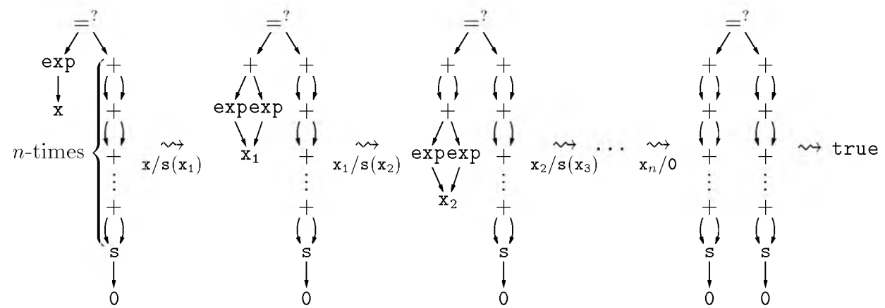
Figure 23: A maximally collapsing narrowing derivation
