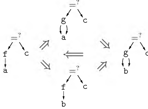
Figure 22: Incompleteness of term graph narrowing
