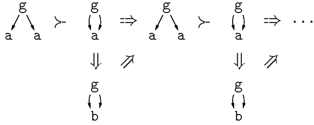
Figure 24: Incompleteness of maximally collapsing narrowing
