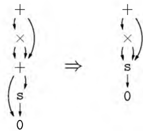
Figure 8: An application of the rule 0 + \mathbf{x} \rightarrow \mathbf{x}
