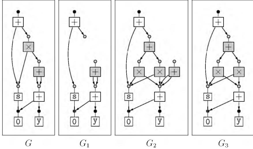
Figure 7: The intermediate steps in the construction of a term graph rewrite step
