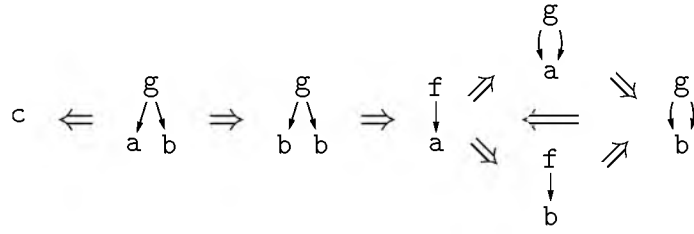
Figure 17: Non-confluence of \Rightarrow and \Rightarrow_{\text{coll}}
