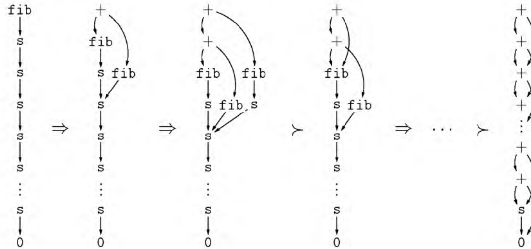
Figure 9: Collapsing to speed up evaluation
