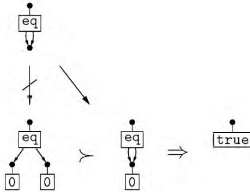
Figure 10: Collapsing to enable a rule application
