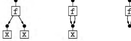
Figure 6: The graphs \Delta f(\mathbf{x}, \mathbf{x}) , \diamond f(\mathbf{x}, \mathbf{x}) and \underline{\diamond f(\mathbf{x}, \mathbf{x})}
