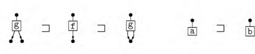
Figure 19: A well-precedence for Example 7.3
