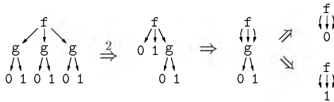
Figure 14: Two terminating derivations
