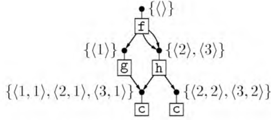
Figure 4: A standard term graph
