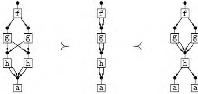
Figure 5: Collapsing and copying
