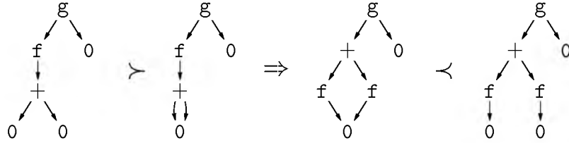
Figure 13: Simulation of a term rewrite step
