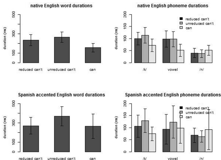
Fig. 1. Mean durations (in ms) of reduced and unreduced can't and of can , and of their phonemes other than /t/, in the stimuli produced by the native speakers of American English (top) and in the stimuli produced by the native speakers of Spanish (bottom, referred to as "Spanish accented English"). The error bars represent one standard deviation.
