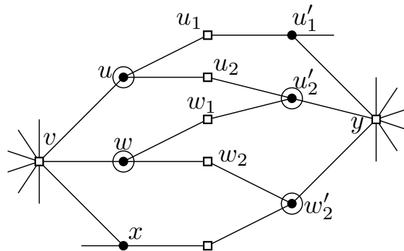
FIG. 4. Illustration of the proof of Claim 2.7. The four removed vertices are circled.
