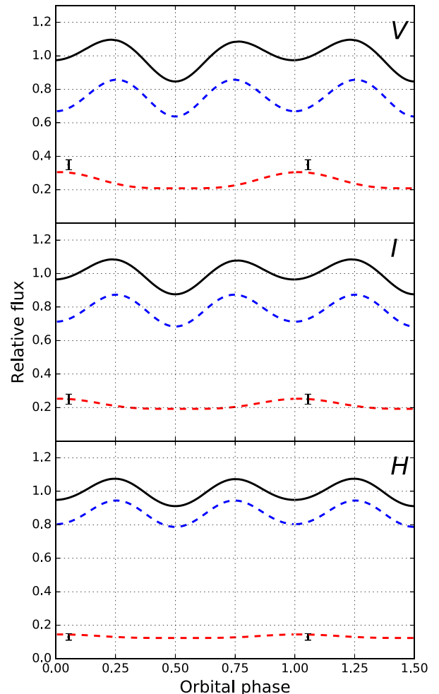
Figure 4. Components of the best-fitting model light curves. Top line: total flux, top dashed line: stellar flux and bottom dashed line: disc flux. The fluxes were normalized such that the orbital average of the total flux is equal to 1.0, corresponding to flux densities of 6.59 \times 10^{27} , 5.64 \times 10^{27} and 1.80 \times 10^{27} \text{ erg s}^{-1} \text{ \AA}^{-1} \text{ sr}^{-1} for V, I and H, respectively. The error bars represent the spectroscopically determined disc fractions of the total flux.
