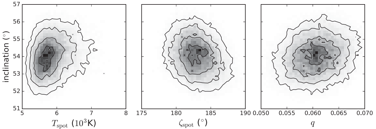
Figure 3. 2D histograms for the MCMC run using all three filter bands, showing the covariance between the orbital inclination and three parameters of the model. Contours enclose approximately 17, 39, 68 and 86 per cent of the samples (corresponding to 0.5, 1.0, 1.5 and 2.0 \sigma for the 1D projections in the case of 2D Gaussian distributions). T_{\text{spot}} and i are positively correlated, as higher disc flux makes the observed fractional ellipsoidal variations smaller than the intrinsic ones. The location of the disc spot \zeta is well-determined, independent of i . The mass ratio q and i are only very slightly interdependent, as expected given the low value of q .
