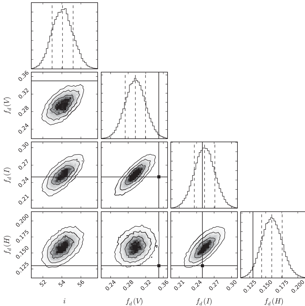
Figure 5. Covariance plots between the orbital inclination and the V , I and H posterior disc fractions (at an orbital phase of 0.054) in the first column, and between the disc fractions in the rest of the figure. These are from the probability distributions resulting from the basic three-band fit. Contours enclose approximately 17, 39, 68 and 86 per cent of the samples (corresponding to 0.5, 1.0, 1.5 and 2.0\sigma for the 1D projections in the case of 2D Gaussian distributions). The dashed lines represent the median values and the 68 per cent most probable interval of each variable. The solid lines indicate the spectroscopically observed values of the latter. The distributions of the V - and H -band deviate significantly from the spectroscopically determined values.
