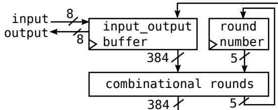
Fig. 4: Round-based architecture
