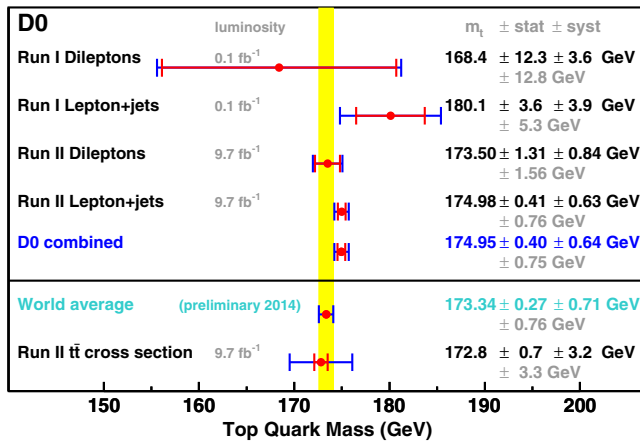
FIG. 2. A summary of the top quark mass measurements used in the D0 combination [9–15], along with the D0 final result, and the top quark pole mass extracted from the D0 cross section measurement [23]. The latter is not used in the combination. The inner red uncertainty bars represent the statistical uncertainties, while the blue bars represent the total uncertainties. For comparison, we also show the preliminary 2014 world average of m_t [20] which includes D0 Run II \ell\ell' and \ell + \text{jets} measurements that are now superseded. For the top quark pole mass extracted from the D0 cross section measurement, a 1.1 GeV theory uncertainty is included in the systematic uncertainty, and the statistical uncertainty is determined such as its relative contribution to the experimental uncertainty is the same as for the cross-section measurement.
