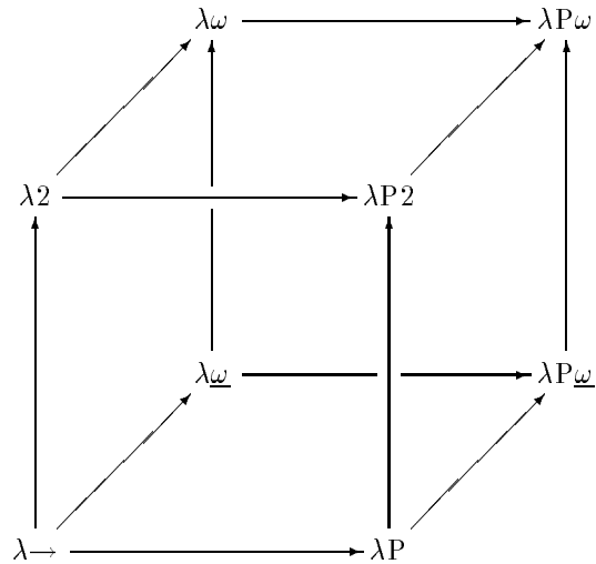
Fig. 2. The \lambda -cube.
