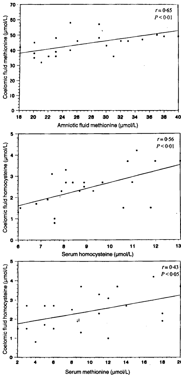
Fig. 3. The correlation coefficients between methionine and total homocysteine in various compartments.
