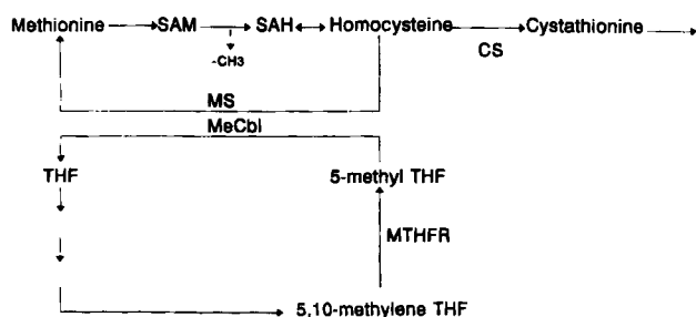
Fig. 1. A simplification of the folate and cobalamin dependent methionine metabolism in humans. CS = cystathionine synthase; MeCbl = methylcobalamin; MS = methionine synthase; MTHFR = methylene THF reductase; SAH = S-adenosylhomocysteine; SAM = S-adenosylmethionine; THF = tetrahydrofolate.
