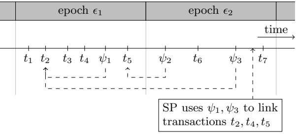
Figure 1: An example of the vote-to-link system with 3 users ( U_1, U_2, U_3 ), 3 moderators ( M_1, M_2, M_3 ) and a threshold k = 2 . The left side of the picture shows how the users and the moderators interact with the service provider: users send transactions ( t_1, \dots, t_7 ) to the service provider. The SP publishes these transactions in a public record after checking their validity. The moderators monitor these transactions, and, whenever they detect a malicious one, send a vote to link to the service provider ( \psi_1, \psi_2, \psi_3 ). The right side of the picture shows a timeline of events at the service provider. After the SP receives k = 2 votes on transaction t_2 , it can link it to the other transactions t_4, t_5 made by the same user in that epoch (note that t_7 is not linked because it was performed in another epoch).
