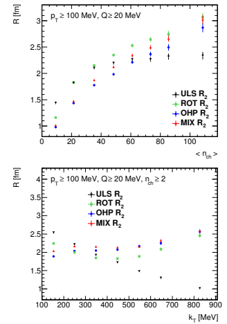
Figure 3. The dependence of R (top) on N and (bottom) on k_t with respect to the beam axis for different reference samples in 7 TeV pp minimum bias events. The exponential parametrization is used [5].
