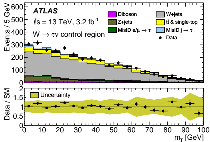
Figure 3: Distribution of m_T in the control region enriched with W \rightarrow \tau\nu events, which differs from the nominal event selection by the requirements that m_T < 100 GeV and that the number of b -tagged jets be zero. The W \rightarrow \tau\nu background is normalised to the data through an overall scale factor. The total (statistical and systematic) uncertainties in the SM prediction are shown in the lower plot.
