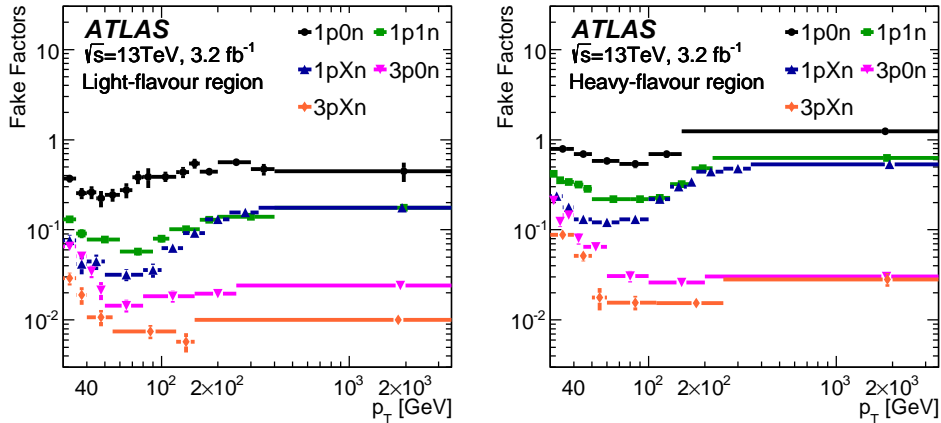
Figure 2: Fake factors parameterised as a function of p_{\text{T}} and the reconstructed \tau_{\text{had}} decay mode, for a b -tagging score of the \tau_{\text{had-vis}} candidate below (left, light-flavour region) or above (right, heavy-flavour region) the chosen threshold. The \tau_{\text{had}} decay mode is referred to as 1p0n, 1p1n, 1pXn, 3p0n or 3pXn, for a p-prong decay with n neutral particles, where X \geq 2 (1) for 1pXn (3pXn) decays. The threshold value for the b -tagging score is set to keep enough entries in each of the two bins, separately for each type of \tau_{\text{had}} decay. The errors shown arise from the statistical uncertainty for a given p_{\text{T}} bin.
