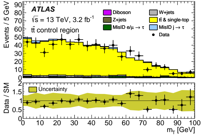
Figure 4: Distribution of m_T in the control region enriched with t\bar{t} events, which differs from the nominal event selection by the requirements that m_T < 100 GeV and that the number of b -tagged jets be at least two. The total (statistical and systematic) uncertainties in the SM prediction are shown in the lower plot.
