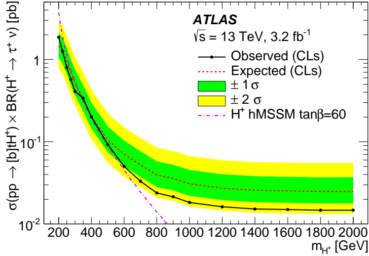
Figure 6: Observed and expected 95% CL exclusion limits for heavy charged Higgs boson production as a function of m_{H^+} in 3.2 \text{ fb}^{-1} of pp collision data. The prediction for \sigma(pp \rightarrow [b]tH^+) \times BR(H^+ \rightarrow \tau\nu) as a function of the charged Higgs boson mass is also shown as a dotted-dashed line, for \tan\beta = 60 in the hMSSM benchmark scenario.
