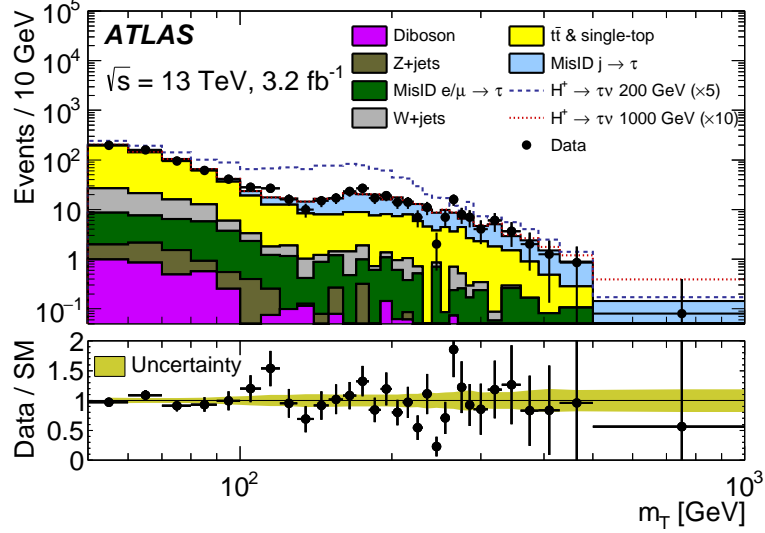
Figure 5: Distribution of m_T after full event selection and a fit to the data with the background-only hypothesis. The horizontal axis starts at m_T = 50 GeV and is in logarithmic scale. Two H^+ signal hypotheses are included on the stack. The signal sample at 200 (1000) GeV is scaled to 5 (10) times the cross section predicted at \tan\beta = 60 in the hMSSM benchmark scenario. Bins are 10 GeV in width up to 310 GeV and then have a varying size. The total (statistical and systematic) uncertainties in the SM prediction are shown in the lower plot.
