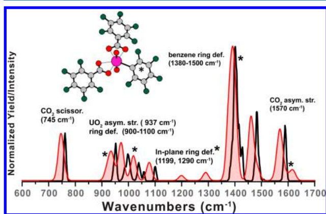
Figure 9. IRMPD spectrum of [(\text{C}_6\text{F}_5)\text{UO}_2(\text{O}_2\text{C}-\text{C}_6\text{F}_5)_2]^- (black). Harmonic frequencies corresponding to the [(\text{C}_6\text{F}_5)\text{UO}_2(\text{O}_2\text{C}-\text{C}_6\text{F}_5)_2]^- GS isomer were computed at the B3LYP/TZ method, scaled by a factor of 0.97 and convoluted with a 25 \text{ cm}^{-1} Gaussian line shape function (red). The computed intensities were normalized to the most intense experimental peak. The computed bands marked with an asterisk correspond to vibrational modes associated with the decarboxylated perfluorophenyl ligand.
