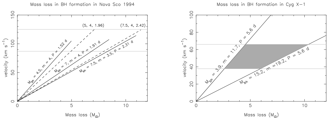
Fig. 1. Limits on the amount of mass ejected in the SN explosion that is required to explain the measured velocities. Left: Nova Sco 1994 with three possibilities of the binary parameters at the onset of the X-ray phase (solid lines; see text) and the two possibilities in the case 0.5 M_{\odot} has been lost draining angular momentum (dashed lines). Right: Cygnus X-1 with two different solutions for the companion mass.
