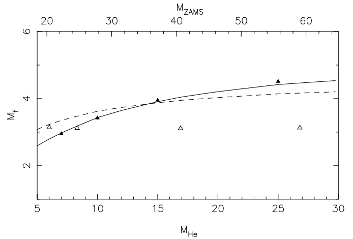
Fig. 3. Final helium star masses as function of the initial helium star mass with the mass-loss rates according to ? , solid line, some of their results are plotted as solid triangles and ? , dashed line assuming a helium star lifetime as given by ? . A selection of their results is plotted as the open triangles. The numbers at the top give an estimate of the ZAMS mass of the progenitor of the helium star.
