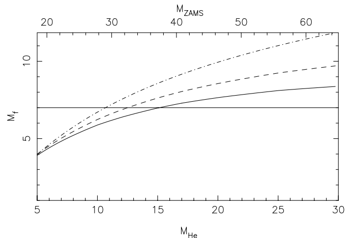
Fig. 4. Final helium star masses as function of initial helium star mass with the mass-loss rates given by Eq. (4) using a helium-star lifetime as given by ? , solid line and the given by ? , dash-dotted line and one with a helium-star lifetime halfway in-between these two (dashed line). ZAMS masses for the helium star progenitors are indicated at the top.
