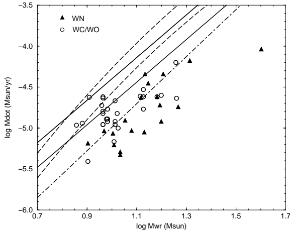
Fig. 2. Mass-loss rates for Wolf-Rayet stars as observed (triangles for WN and circles for WC/WO stars, from ? , where we excluded the hydrogen rich Wolf-Rayet stars) and various relations used for evolutionary calculations. The solid lines are the relations assumed by ? for WC (upper) and WN (lower) stars. The dashed lines are the ones used by ? , where we converted the mass loss – luminosity relations to mass loss - mass relations using the mass - luminosity relation of ? . The upper dashed line is for their standard case, the lower for their reduced mass loss case. The dash-dotted line is a rectangular least square fit to all points (see also the text and Eq. (4)).
