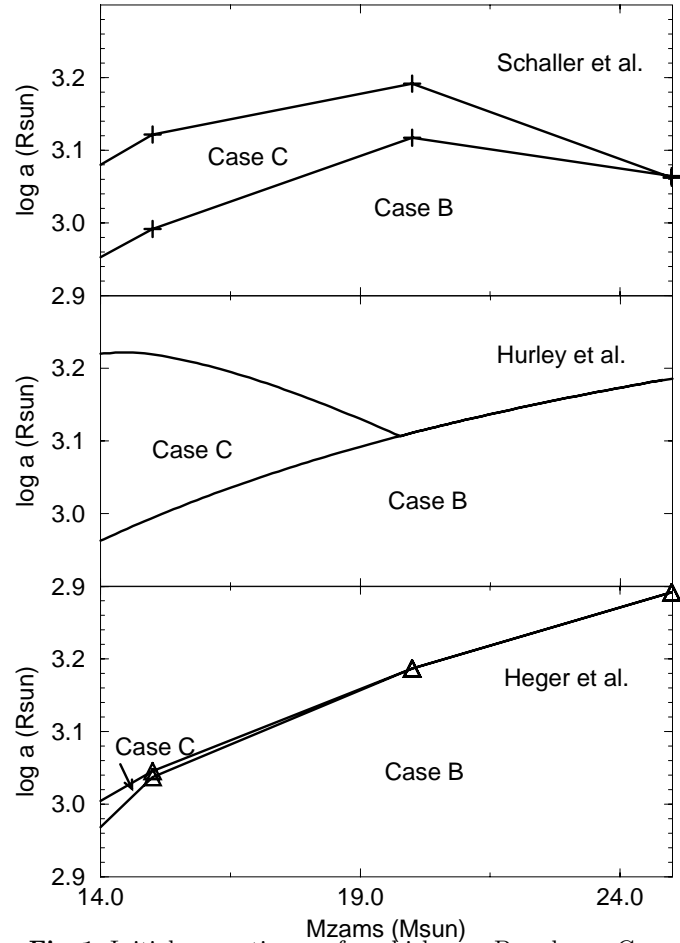
Fig. 1. Initial separations a_i for which case B and case C mass transfer occur as function of ZAMS mass, for a 1 M_{\odot} companion. Top for the ? models, middle for the ? models, bottom for the ? models.
