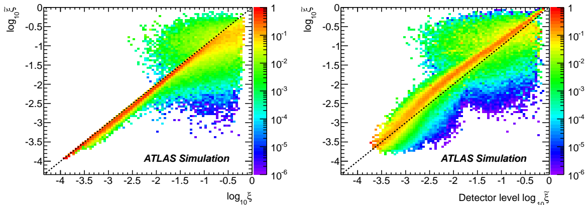
Figure 2: (a) Particle-level correlation between the \xi variable extracted from the diffractively scattered proton and \tilde{\xi} calculated from particles selected as defined in the text, using the PYTHIA8 SD MC model. (b) Correlation between the particle-level \tilde{\xi} and detector-level \tilde{\xi} calculated from clusters selected as defined in the text, using the sum of PYTHIA8 ND, SD and DD contributions. In both plots, the distributions are normalised to unity in each column.
