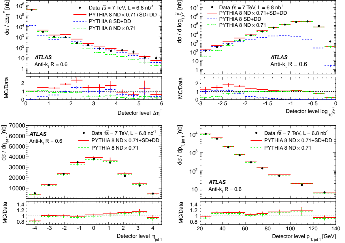
Figure 3: Comparisons of dijet cross sections from uncorrected data with a combination of PYTHIA8 diffractive and non-diffractive contributions at detector level based on jets found by the anti- k_t algorithm with R = 0.6 . The MC distributions are normalised to the integrated luminosity of the data after first applying a factor of 0.71 to the ND contribution. The error bars correspond to the statistical uncertainties. In addition to the measured (a) \Delta\eta^F and (b) \tilde{\xi} variables, the distributions in (c) the leading-jet pseudorapidity and (d) transverse momentum are also shown. The lower panels show ratios of the MC models to the data where the error bars indicate the sum in quadrature of the statistical uncertainties arising from the data and the MC simulation.
