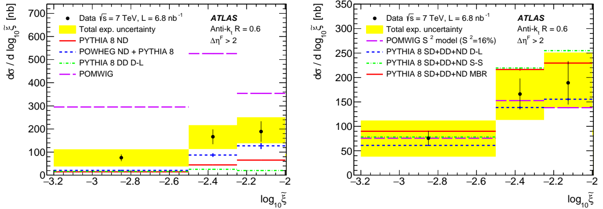
Figure 6: The differential cross section as a function of \tilde{\xi} for events satisfying \Delta\eta^F > 2 . The same data are shown in (a) and (b), and are compared with models as described in the text. The error bars on the data and the MC models indicate their respective statistical uncertainties, while the yellow bands show the total uncertainties on the data. The 'POMWIG S^2 ' model represents the sum of PYTHIA ND and POMWIG, with POMWIG multiplied by 0.16 and scaled by 1/1.23 and by the (SD+DD)/SD ratio from PYTHIA8.
