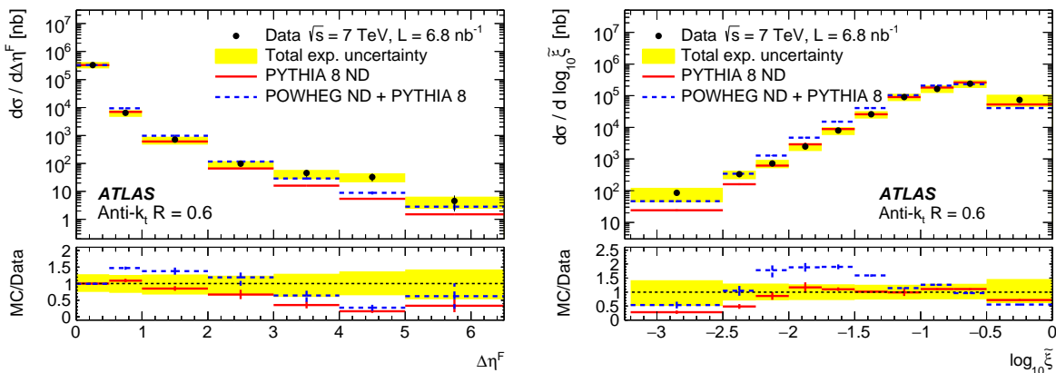
Figure 5: The dijet cross sections differential in (a) \Delta\eta^F and (b) \tilde{\xi} , compared with the PYTHIA8 ND MC model as well as an ND model using the NLO POWHEG generator with hadronisation based on PYTHIA8. Each of the models is separately normalised to match the data in the first \Delta\eta^F bin. The error bars on the data and the MC models indicate their respective statistical uncertainties, while the yellow bands show the total uncertainties on the data. The lower panels show ratios of the MC models to the data where the error bars indicate the sum in quadrature of the statistical uncertainties arising from the data and the MC simulation.
