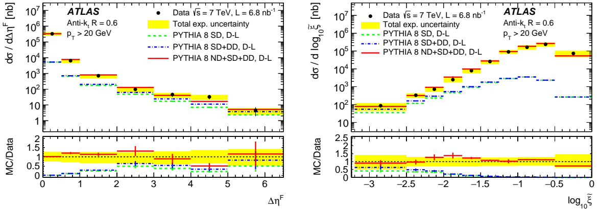
Figure 4: The differential dijet cross sections in (a) \Delta\eta^F and (b) \tilde{\xi} , compared with the particle-level PYTHIA8 model of the SD, sum of diffractive components SD and DD, and sum of all three ND, SD and DD components. The Donnachie–Landshoff pomeron flux model is used for the diffractive components. The error bars on the data and the MC models indicate their respective statistical uncertainties, while the yellow bands show the total uncertainties on the data. The ND contribution is normalised to match the data in the first \Delta\eta^F bin. The lower panels show ratios of the MC models to the data where the error bars indicate the sum in quadrature of the statistical uncertainties arising from the data and the MC simulation.
