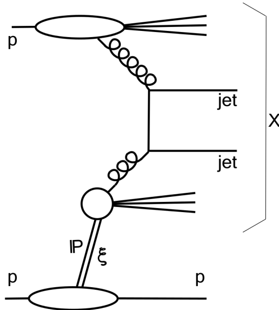
Figure 1: Illustration of hard single-diffractive scattering, in which partons from a pomeron (IP) and from a proton enter a hard sub-process. The rapidity gap appears between the system X and the intact proton.
