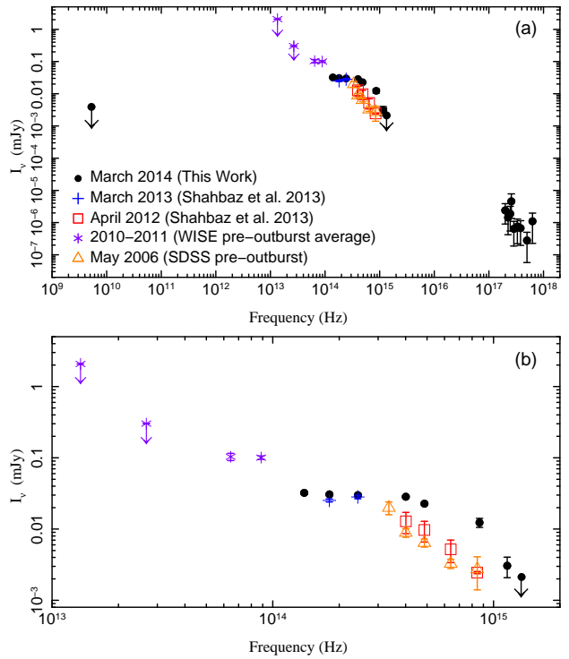
Figure 4. Broadband spectrum of J1357.2 with archival IR, NIR, and optical observations. Black circles are data from our 2014 quiescent campaign (repeated from Figure 3). Other symbols denote NIR and optical data at previous epochs (as published by Shahbaz et al. 2013), pre-outburst optical data from the SDSS, and pre-outburst IR observations from WISE (see legend for details). For clarity, panel (b) shows a zoom-in of the IR–UV portion of the spectrum.
