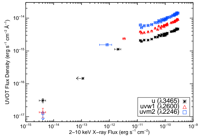
Figure 2. The UV/X-ray luminosity correlation for J1357.2. The UV filters (from Swift/UVOT) and their effective wavelengths are noted in the legend. Hard state data is taken from Armas Padilla et al. (2013) during the 2011 outburst decay (we only include filters for which we have quiescent observations), and the data points at the lowest X-ray flux are from our recent campaign in quiescence. The shape of the UV spectrum changes in quiescence and becomes redder (i.e., steeper).
