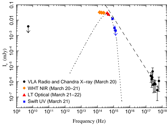
Figure 3. Broadband quiescent spectrum of J1357.2 from our quasi-simultaneous multiwavelength campaign in March 2014. Data points are coded by date of observation (see legend for details). Chandra data are unfolded, binned to >2 counts per bin. We also show our best-fit X-ray power-law spectrum ( \Gamma = 2.6 ; dashed line) extrapolated to lower frequencies, and a blackbody curve ( T_{\text{bb}} = 7000 \pm 300 K) that fits the optical/UV data (dotted line). We illustrate the X-ray spectrum with the best-fit \Gamma = 2.6 instead of the canonical \Gamma = 2.1 adopted elsewhere in the paper, in order to more conservatively illustrate that the UV spectrum is steeper than the X-ray spectrum.
