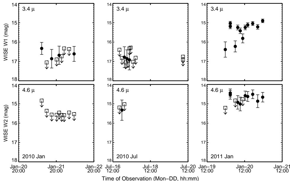
Figure 5. Pre-outburst IR light curves of J1357.2 in the WISE W1 (top row) and W2 (bottom row) filters. Observations taken during 2010 January, 2010 July, and 2011 January are shown in the left, middle, and right columns, respectively. Filled circles with error bars illustrate detections, while open squares represent 95% lower limits on the magnitude. The 2011 January observations were taken only eight days before J1357.2 was discovered in outburst in the X-ray, indicating that the outburst rise timescale was \lesssim 1 week.
