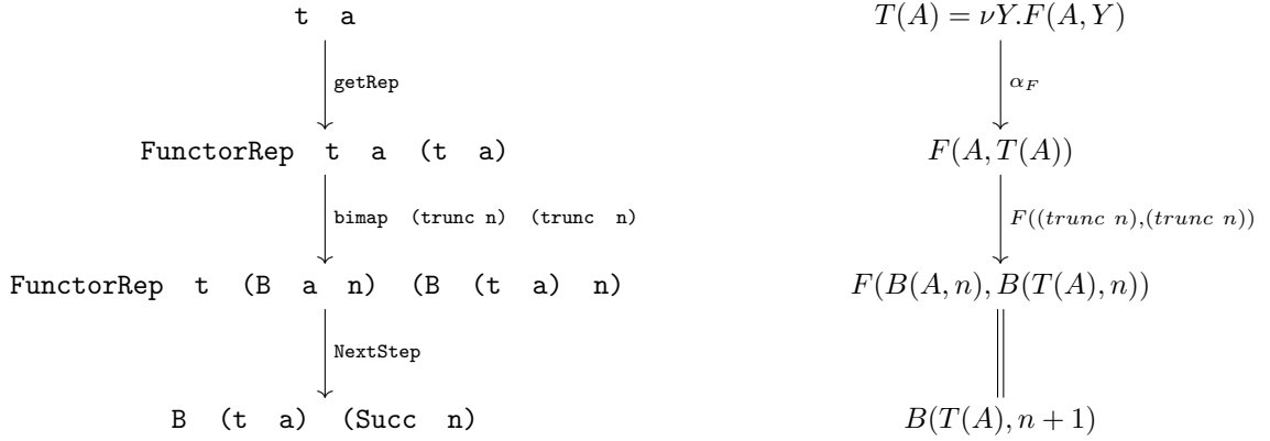
■ Figure 2 Generic definition of truncations in Haskell.
