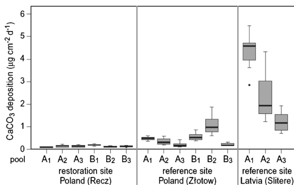
Fig. 3 Box plots of \text{CaCO}_3 deposition in \mu\text{g Ca}^{2+} \text{cm}^{-2} \cdot \text{d}^{-1} measured on microscope slides ( n = 8 per pool) in experimental pools in Polish and Latvian spring mires. The boxes (Tukey boxplot) comprise of the 25 % quartile, the median (solid black line) and the 75 % quartile. Whiskers represent data within 1.5 times the interquartile range from the box. Data outside the whiskers are respectively higher or lower.
