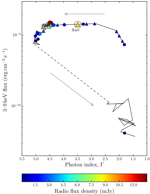
Figure 4. Proxy Swift Hardness–Intensity diagram (photon index versus flux) of the outburst, superimposed with 5.25 (circle) and 15.7 GHz (triangle) radio flux densities, with arrows representing temporal direction. The dashed line represents the period when X-ray observations were unavailable due to the source being Sun-constrained. The radio flux peaked in the soft (or possibly, late-intermediate) state while the sharp 15.7 GHz radio flare at MJD 56602 (circled) occurred during the intermediate state.
