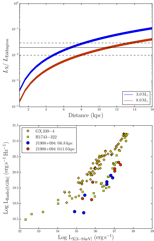
Figure 6. Upper panel: Assuming that the source transitions from a soft to hard state at 2% of the Eddington luminosity and a representative black hole mass of 8 M_{\odot} (Kreidberg et al. 2012), the observed fluxes imply a source distance of 11 kpc (red), or, for a black hole mass of 3 M_{\odot} , 6.8 kpc (blue). Width of lines corresponds to uncertainty in observed flux at the state transition observed in 2002. Solid and dashed lines represent 2, 1 and 3 % of the Eddington luminosity. Lower panel: The hard-state X-ray–radio luminosity correlation shows representative data from the upper (GX 339–4; Corbel et al. 2013) and lower (H1743–322; Coriat et al. 2011) branches, overlaid by our data for XTE J1908+094 at assumed distances of 6.8 kpc and 11 kpc (the latter distance being more consistent with the representative data).
