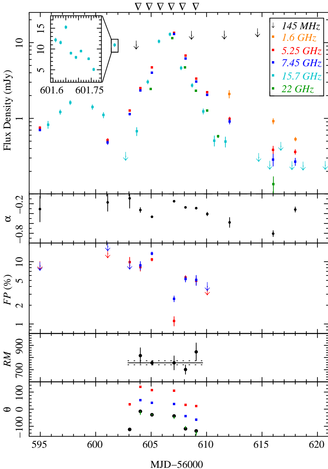
Figure 2. Radio light curves, spectral, and polarisation parameters of the source during outburst. The upper panel shows the flux densities at each of the 6 radio frequencies observed (legend is common to all panels), while the inlay shows the time-resolved 15.7 GHz data from MJD 56601.7. The second panel shows the radio spectral index, \alpha (where F_\nu \propto \nu^\alpha ), while the third panel shows the fractional polarisations or limits, FP , at 2 frequencies (5.25 and 7.45 GHz; note that for clarity we only plot constraining limits, i.e., \leq 20\% ). The fourth panel shows the rotation measure, RM , from independent (data points) and simultaneous (solid line with 1\sigma errors as dashed lines) fitting of the epochs. Panel five shows the observed polarisation angles (blue and red) and the intrinsic electric vector position angle (EVPA), \theta , derived from the independent (green) and simultaneous (black) fits of those PAs. The inverted triangles along the top
