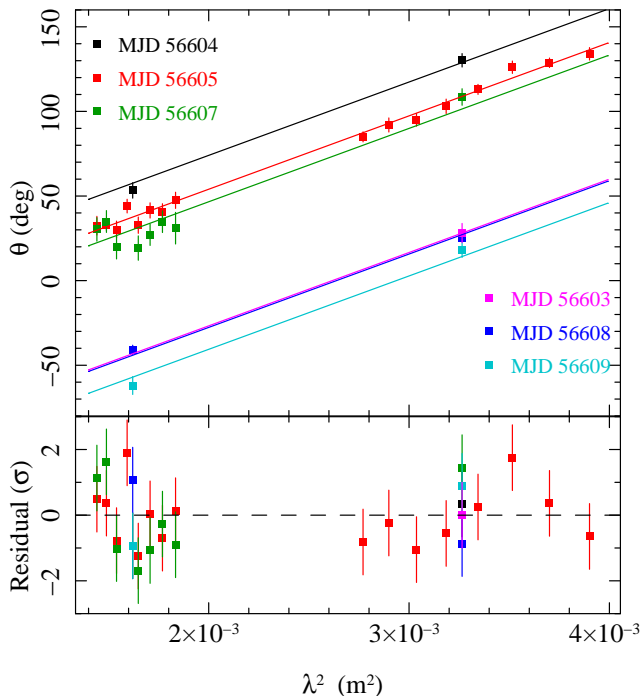
Figure 3. Plot of observed polarisation angle versus wavelength, and simultaneous fit for the rotation measure, for the 6 epochs with observed polarisations. The lower panel shows the residuals (in units of \sigma ) from the simultaneous fit.
