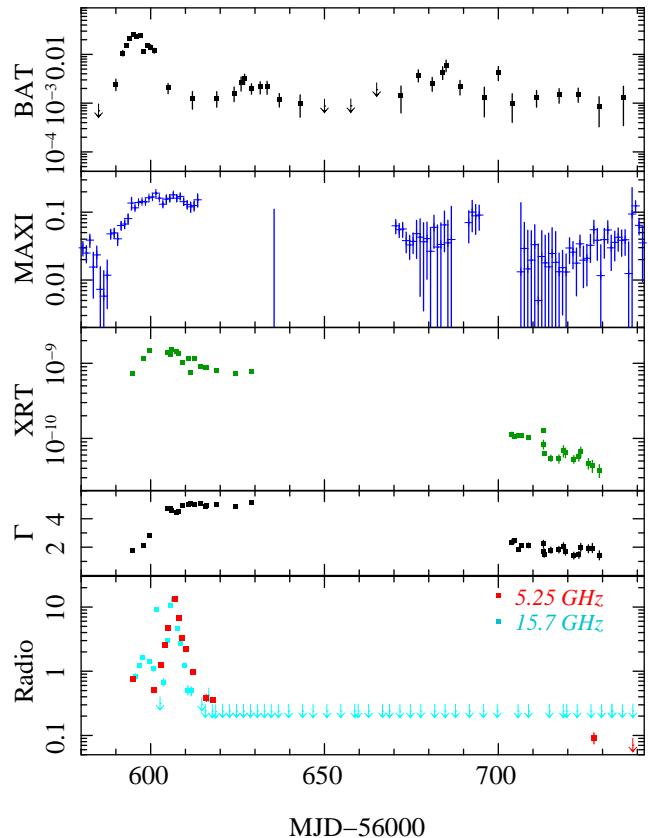
Figure 1. Hard Swift /BAT 15–50 keV, counts/second) and soft (MAXI 2–20 keV, counts/second 6 ; Swift /XRT 3–9 keV, \text{ergs cm}^{-2} \text{s}^{-1} ) X-ray light curves, X-ray photon index ( \Gamma ), and radio (5.25 GHz & 15.7 GHz, mJy) light curves. Due to the source’s proximity to the bright, persistent source GRS 1915+105, MAXI count-rates may suffer from contamination, especially at low luminosities.
