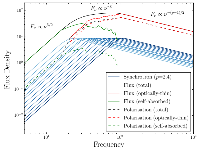
Figure 5. Schematic representation of the flux and polarisation from a compact, partially self-absorbed jet demonstrating that the polarisation of the flat spectrum is dominated by optically-thin regions. The underlying distribution of the electron populations producing the individual synchrotron spectra is arbitrary, as are the flux and frequency units.
