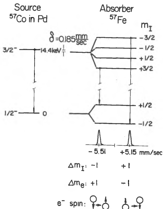
FIG. 1. Energy-level diagram of 57 Fe, indicating the \Delta m_I = 1 transitions, and the corresponding changes in angular momentum of the internally converted electrons.
