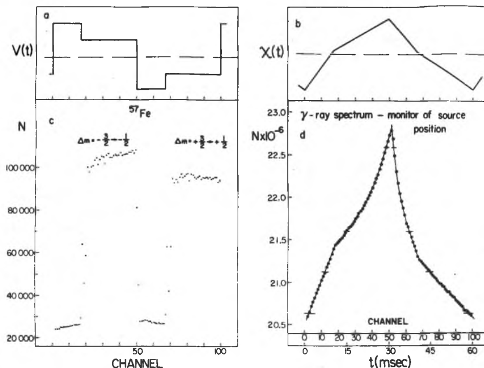
FIG. 2. (a) Reference wave form applied to the source drive, (b) corresponding source displacement, (c) electron spectrum obtained with the electron spectrometer set for detection of K electrons (total measuring time for this run was 89 h), and (d) spectrum of nonresonant radiation scattered from the absorber; channel intervals having the same source position are indicated by horizontal bars.
