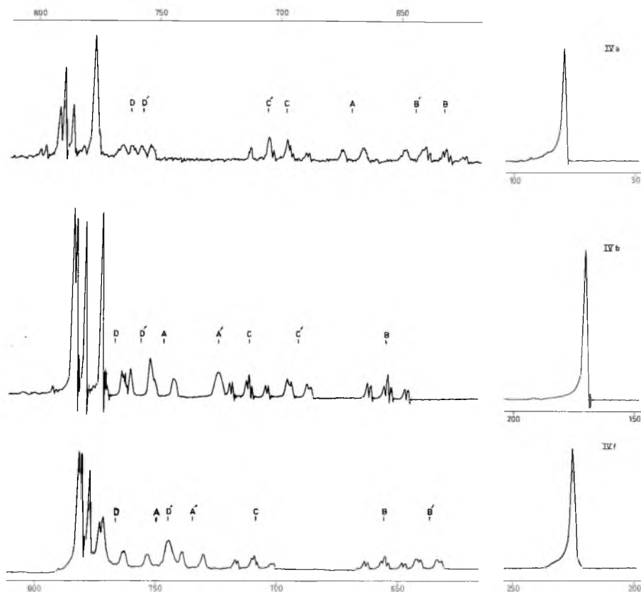
FIG 1. NMR spectra of 1-methyl-(IVa); 2-methyl-(IVb) and 3-methylhexahelicene (IVc) in \text{CS}_2 solution (100 Mc/s)
