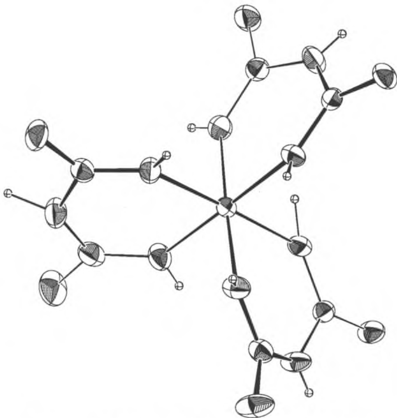
Fig. 1. Projection of the anion along the a^* axis on the bc plane, showing the anisotropic vibration ellipsoids. The hydrogen positions are very inaccurate ( \text{esd} = 0.2 Å).
