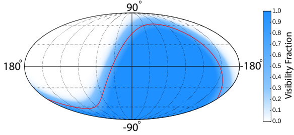
Figure 3: The angular coverage in Galactic coordinates. The color scale represents the fraction of livetime that a patch of the sky is visible. The solid line shows the sky visible to a detector at the South Pole.
