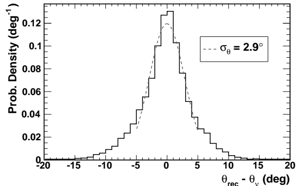
Figure 7: The angular difference between the reconstructed and true neutrino direction in the local zenith direction. A resolution of \sigma_\theta = 2.9^\circ is found for an eight-antenna ARIANNA station. Figure adapted from Ref. [43].
