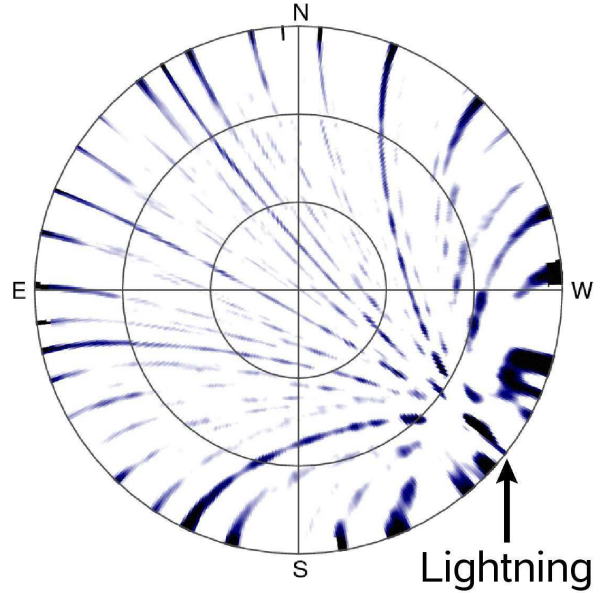
Fig. 6. Sky map of the thunderstorm event shown in Fig. 5 [28].
