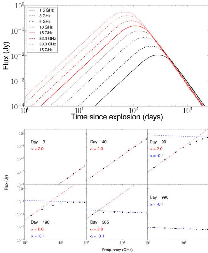
Figure 1. Top: synthetic radio light curves for a spherical eruption at a distance of 1 kpc, M_{ej} = 1 \times 10^{-4} M_{\odot} , V_{max} = 3000 \text{ km s}^{-1} , T_e = 17,000 \text{ K} , and the ratio of the inner to outer radius of the shell of 0.25. The different frequency colors and line styles are as in the labels and Table 1. Bottom: spherical-model spectral evolution at different dates demonstrating how the spectral index changes from completely optically thick ( \alpha = 2.0 ) to thin ( \alpha = -0.1 ). Furthermore, to guide the eye, lines are drawn to show the evolution of the spectral index from completely optically thick to thin.
