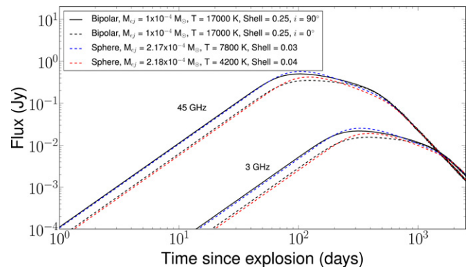
Figure 5. Best-fit spherical-model synthetic light curves are fitted to bipolar-model synthetic light curves. The input bipolar model at 0^\circ and 90^\circ (dashed and solid black lines, respectively) assumes M_{\text{ej}} = 1 \times 10^{-4} M_{\odot} , T_e = 17,000 K, V_{\text{max}} = 3000 km s ^{-1} , and a relative shell thickness of 0.25 at a distance of 1 kpc. The best-fit spherical models are shown as blue and red dashed lines for the bipolar models at 90^\circ and 0^\circ , respectively. The result shows that to find the best fit while keeping the maximum expansion velocity and distance constant, we require that the ejected mass double increase the shell size (so that it reaches closer to the explosion site), and, depending on the inclination, reduce the temperature by more than half.
