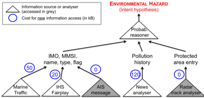
Figure 2. METIS information retrieving and processing components as a definite stratified multi-context system.
