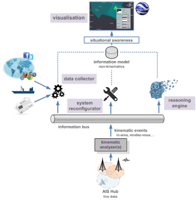
Figure 4. The general architecture of the METIS system.
