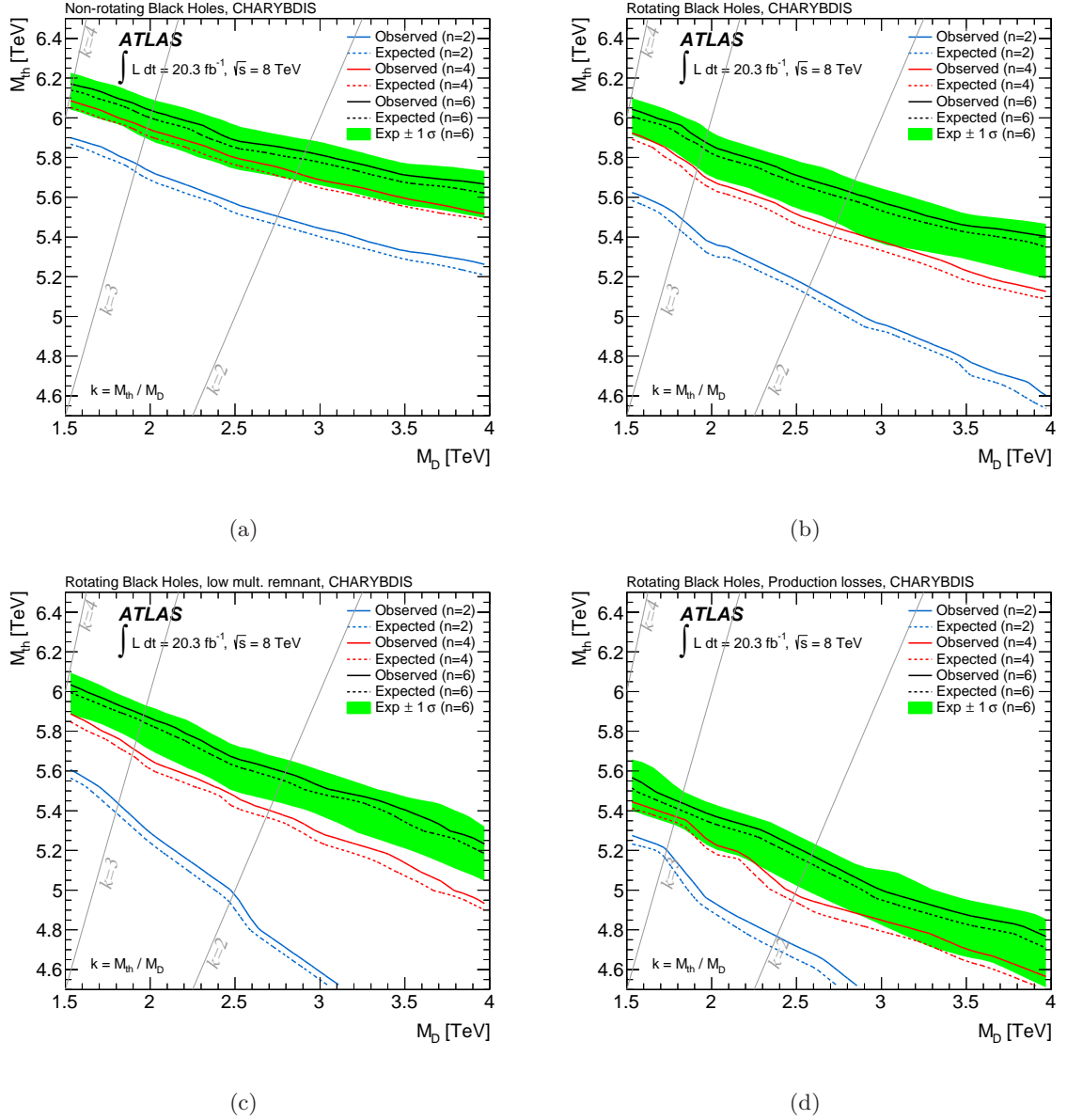
Figure 8. The exclusion limits in the M_{\text{th}} - M_{\text{D}} plane, with electron and muon channels combined, for (a) non-rotating and (b) rotating black hole models in two, four and six extra dimensions, simulated with CHARYBDIS. The lower panes show limits for (c) rotating black holes with low multiplicity remnant decays and (d) with production phase losses turned on. The solid (dashed) lines show the observed (expected) 95% CL limits, with the shaded band illustrating the expected \pm 1 \sigma variation of the n = 6 expected limits. The \pm 1 \sigma variation is comparable for the n = 2 and n = 4 models. Masses below the corresponding lines are excluded. The lighter grey lines indicate constant k = M_{\text{th}} / M_{\text{D}} .
