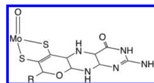
Figure 1. Mo center with one of two coordinating ene-dithiolate pyranopterin cofactors present in mononuclear Mo enzymes.
