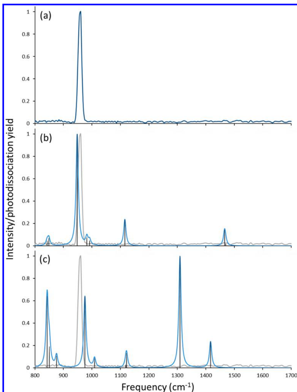
Figure 6. (a) Experimental IRMPD and (b and c) predicted spectra for [\text{MoO}(\text{mnt})_2]^{2-} . Theoretical frequencies were generated at the B3LYP/6-311+G(d) level of theory and are scaled by a factor of 0.96. The predicted spectrum in (b) is for a doublet spin state, while the one in (c) is for a quartet spin state.
