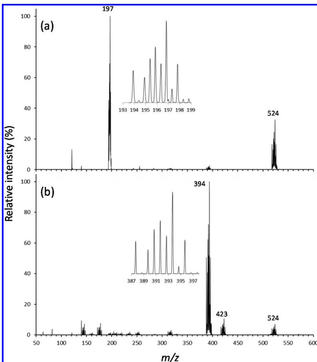
Figure 3. ESI mass spectra generated from acetonitrile solution of [\text{MoO}(\text{mnt})_2]^{2-} as the tetraethylammonium salt: (a) conditions optimized for production of doubly charged anion and (b) conditions retuned for optimized yield of the oxidized species [\text{MoO}(\text{mnt})_2]^- . The insets are high-resolution scans to show the expected Mo isotope patterns for the two ions.
