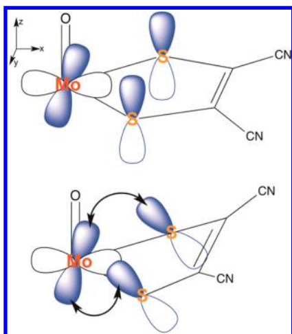
Figure 2. Depiction of ligand “folding” proposed to modulate electron transfer in mononuclear molybdenum enzymes.
