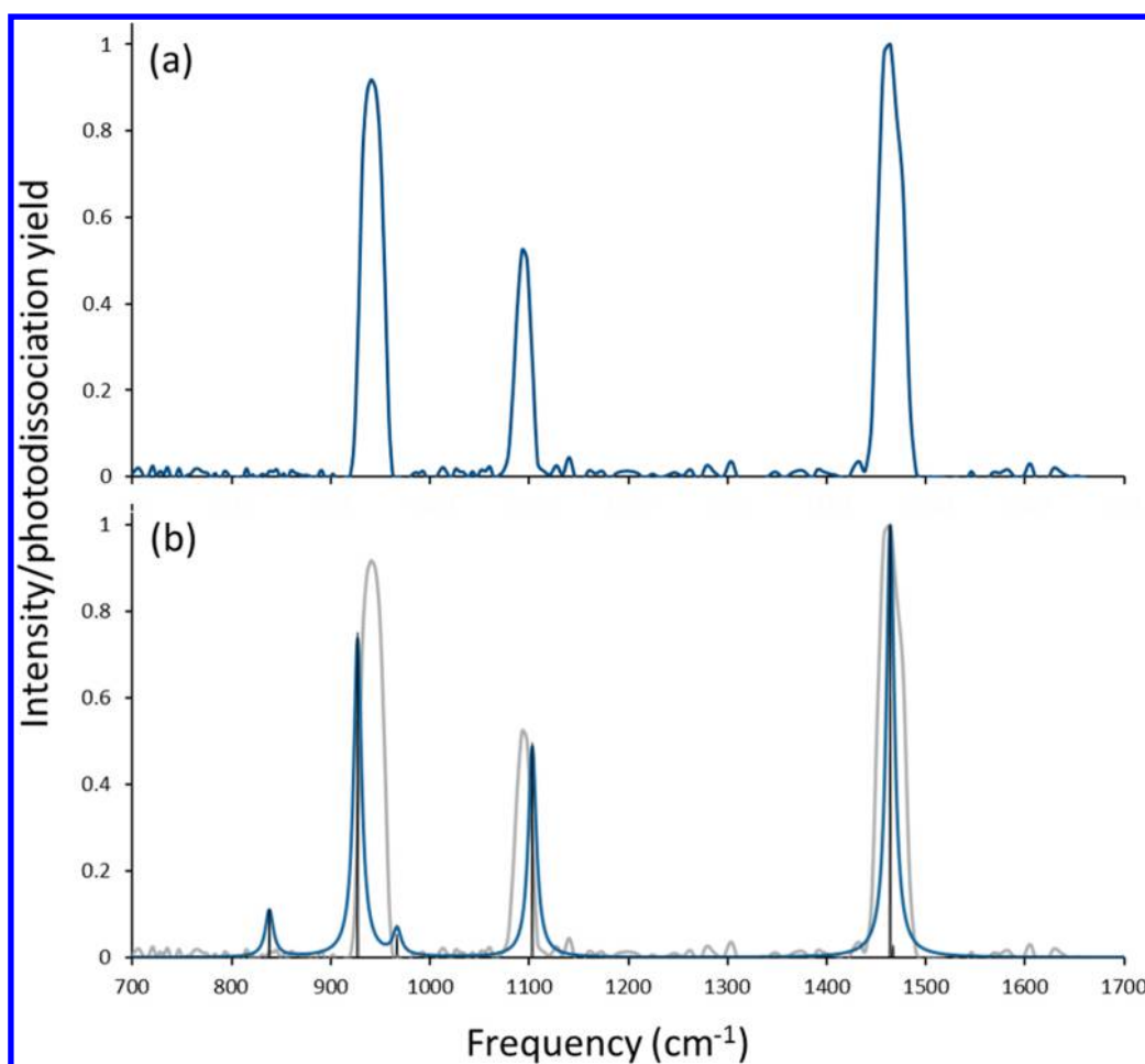
Figure 5. (a) Experimental IRMPD and (b) predicted spectra for [\text{MoO}(\text{mnt})_2]^{2-} . Theoretical frequencies were generated at B3LYP/6-311+G(d) level of theory using a singlet spin state and are scaled by a factor of 0.96.
