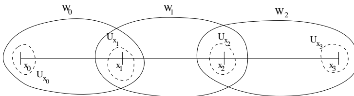
Figure 1: A subdivision of \theta with n = 3 .
