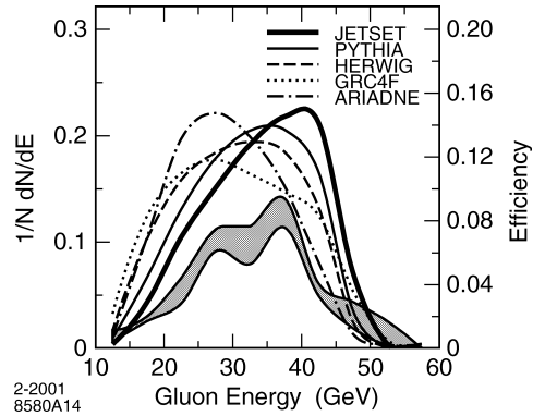
Fig. 3. Energy distribution (left-hand scale) of gluons for the g \rightarrow b\bar{b} process in different models (see text). Our calculated efficiency and its uncertainty (see text) are shown as the band (right-hand scale).
