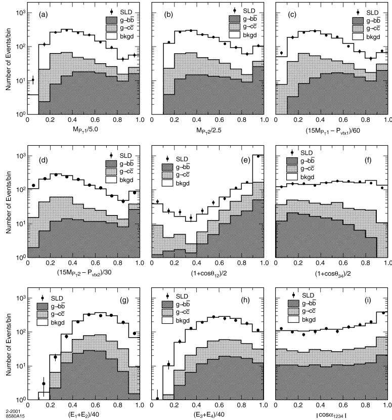
Fig. 1. Distribution of M_{P_T1} (see text). The right-most bin includes overflows. The points represent the data, the histogram the simulation; the expected contribution from g \rightarrow b\bar{b} ( g \rightarrow c\bar{c} ) (see text) is shown as the dark (shaded) area.
