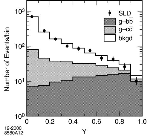
Fig. 2. Distribution of the neural network output Y . The points represent the data, the histogram the simulation; the expected contribution from g \rightarrow b\bar{b} ( g \rightarrow c\bar{c} ) (see text) is shown as the dark (shaded) area.
