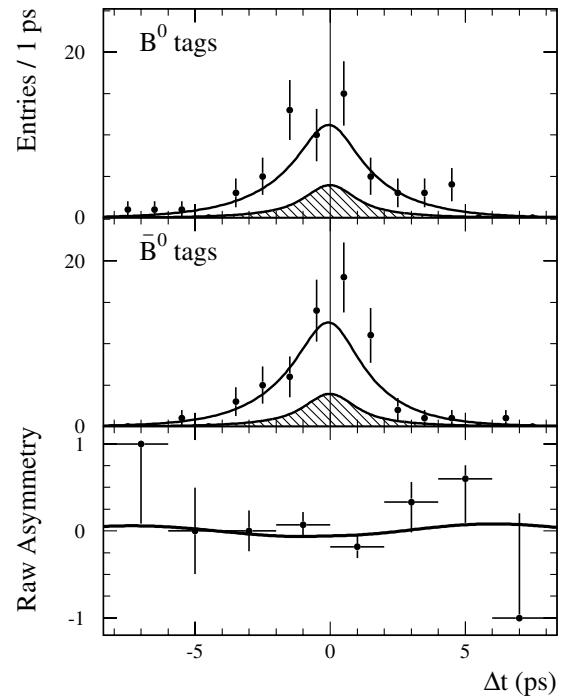
FIG. 2. From top to bottom: Number N_{B^0} ( N_{\bar{B}^0} ) of candidate events in the region m_{\text{ES}} > 5.27 \text{GeV}/c^2 with a B^0 ( \bar{B}^0 ) tag, and the raw asymmetry (N_{B^0} - N_{\bar{B}^0})/(N_{B^0} + N_{\bar{B}^0}) , as functions of \Delta t . The solid curves represent the result of the combined fit to the full sample. The shaded regions represent the background contributions.
