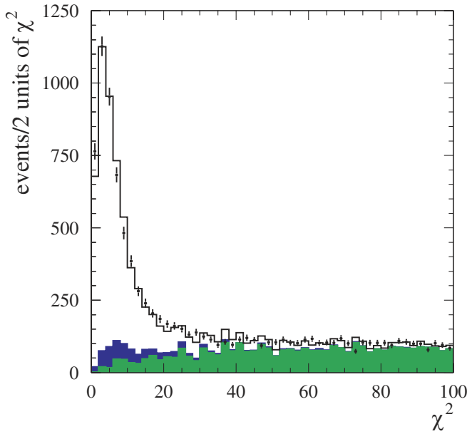
FIG. 4 (color online). The \chi^2 distribution for events from the mass range 1.05 < M_{3\pi} < 3.00 GeV/ c^2 after background suppression cuts. The points with error bars show the data distribution. The histogram is the sum of simulated distributions for e^+e^- \rightarrow \pi^+\pi^-\pi^0\gamma and background processes. The dark and lightly shaded histograms show the distributions for e^+e^- \rightarrow \pi^+\pi^-\pi^0\pi^0 and other background processes, respectively.
