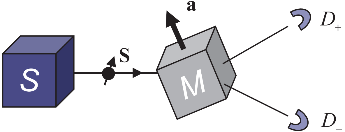
Figure 2: (Color online) Diagram of the Stern-Gerlach experiment. The source S , activated at times labeled by n = 1, 2, \dots, N , sends a particle carrying a magnetic moment \mathbf{S} to the magnet M with its magnetization in the direction \mathbf{a} . Depending on the relative directions of \mathbf{a} and \mathbf{S} , the particle is detected with 100% certainty by either D_+ or D_- .
