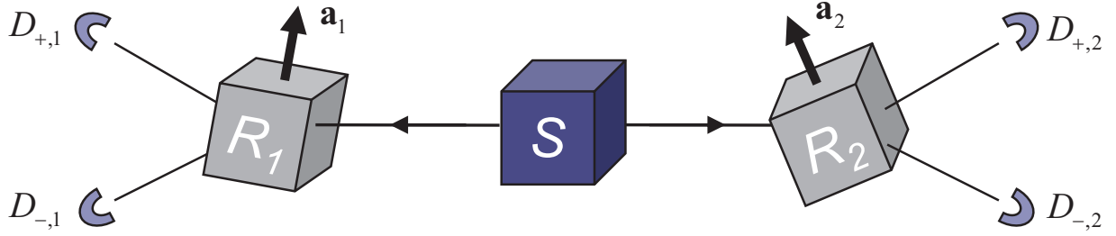
Figure 1: (Color online) Diagram of the EPRB thought experiment. The source S , activated at times labeled by n = 1, 2, \dots, N , sends a signal to the router R_1 and another signal to the router R_2 . Depending on the orientations of the routers, represented by unit vectors \mathbf{a}_1 and \mathbf{a}_2 , the signal going to the left (right) is detected with 100% certainty by either D_{+,1} or D_{-,1} ( D_{+,2} or D_{-,2} ).
