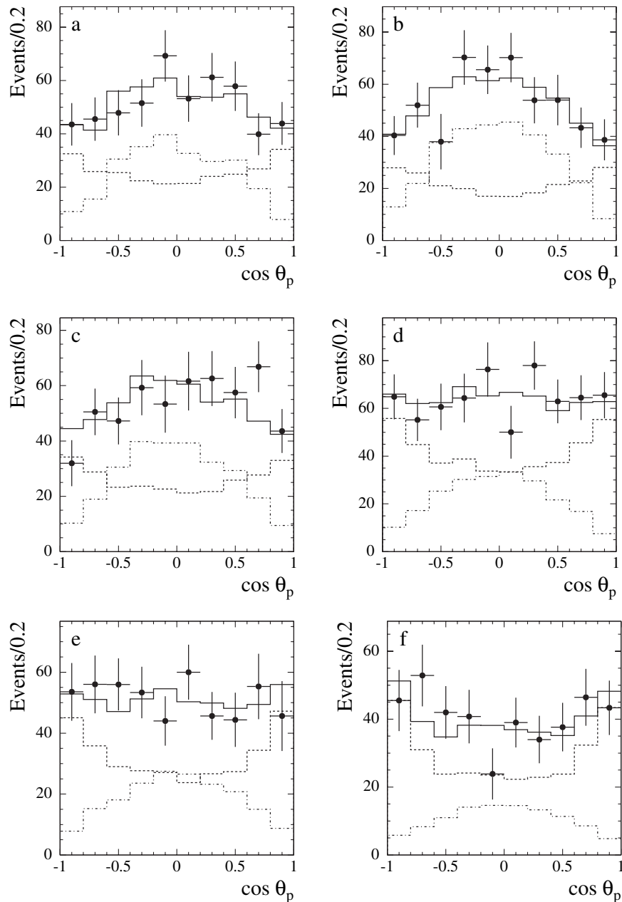
FIG. 9. The \cos\theta_p distributions for different p\bar{p} mass regions: (a) 1.877–1.950 \text{GeV}/c^2 , (b) 1.950–2.025 \text{GeV}/c^2 , (c) 2.025–2.100 \text{GeV}/c^2 , (d) 2.100–2.200 \text{GeV}/c^2 , (e) 2.200–2.400 \text{GeV}/c^2 , (f) 2.400–3.000 \text{GeV}/c^2 . The points with error bars show data distributions after background subtraction. The histograms are fit results: the dashed histograms show the contributions corresponding to the magnetic form factor; the dash-dotted histograms show the contributions from the electric form factor.
